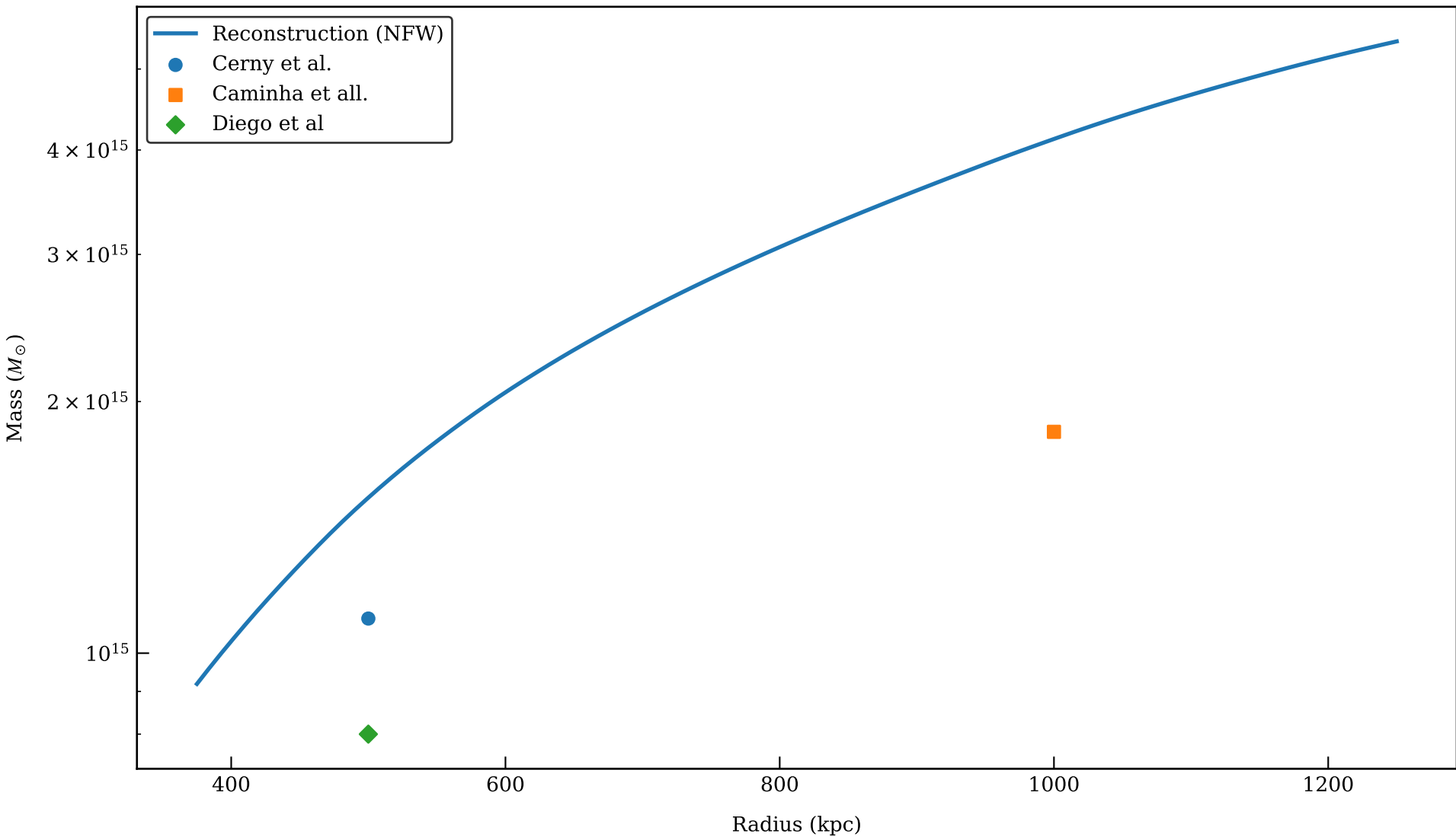
Mass Comparison: EL_GORDO (NFW, signals: shear_g)
