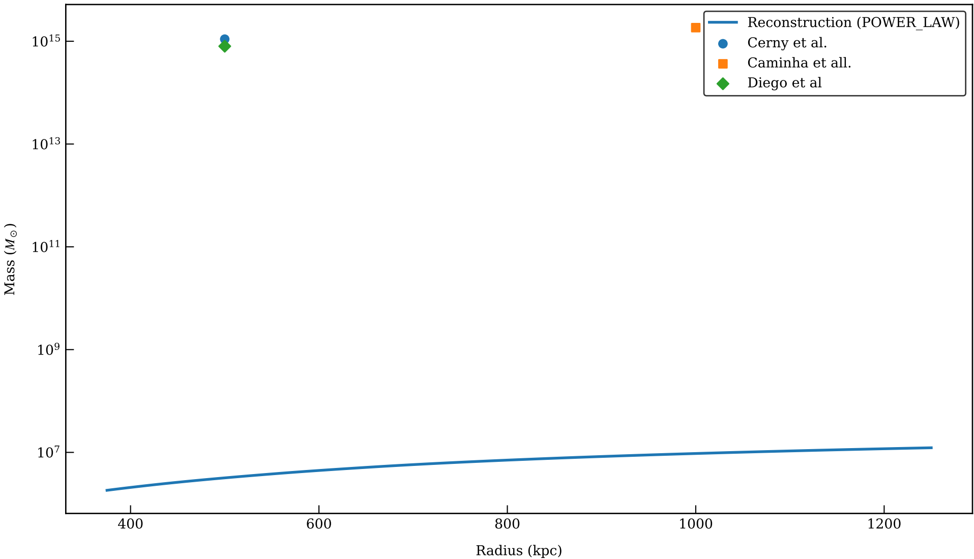
Mass Comparison: EL_GORDO (POWER_LAW, signals: shear_g)
