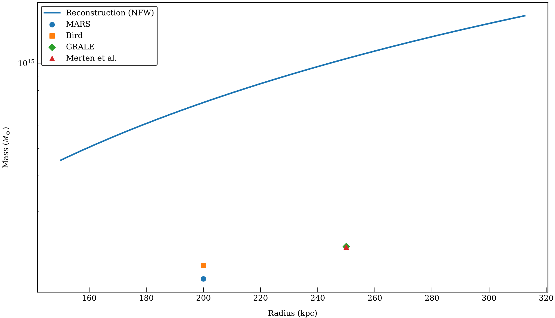
Mass Comparison: ABELL_2744 (NFW, WL+SL, signals: f_g)
