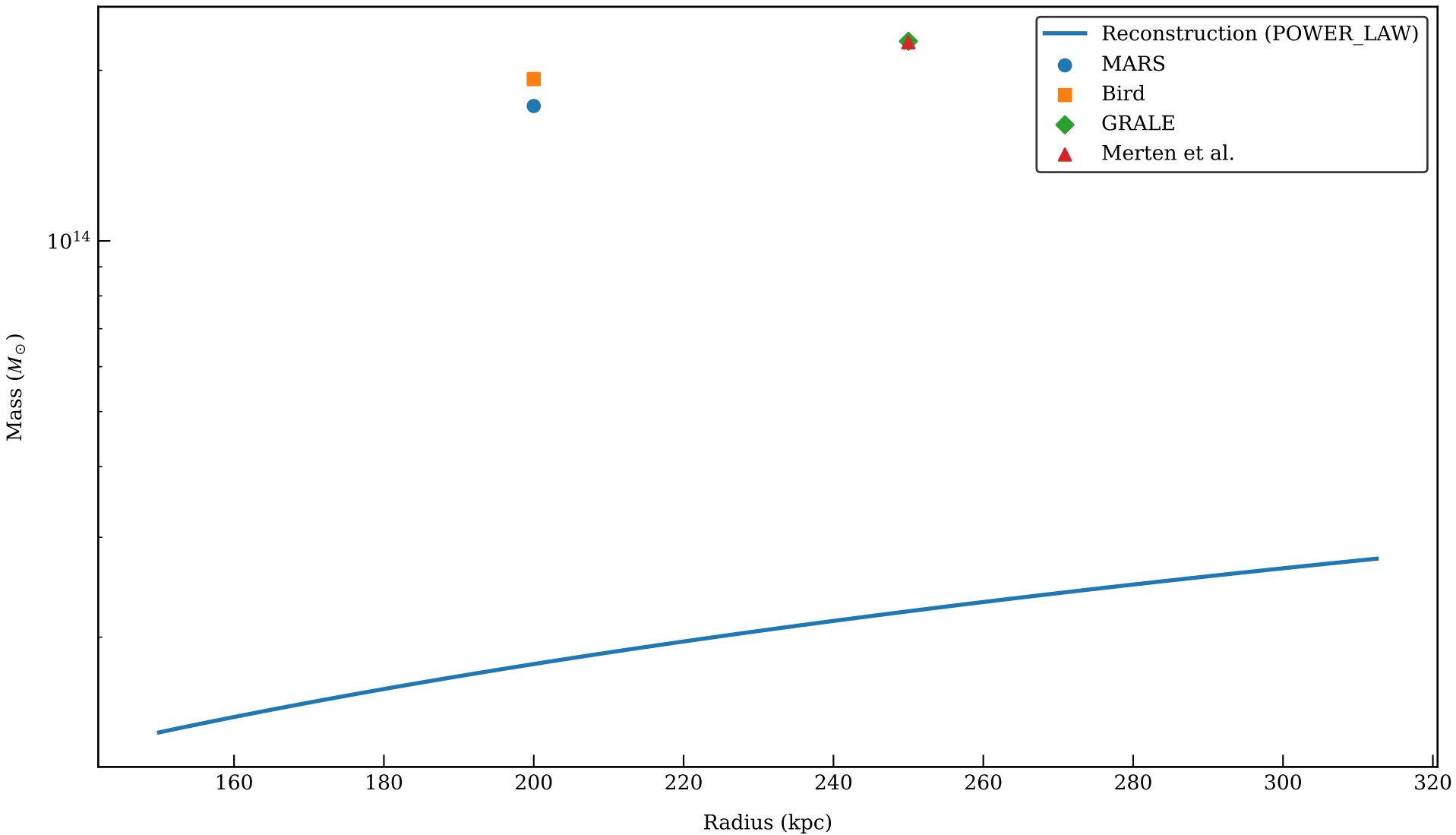
Mass Comparison: ABELL_2744 (POWER_LAW, WL+SL, signals: f_g)
