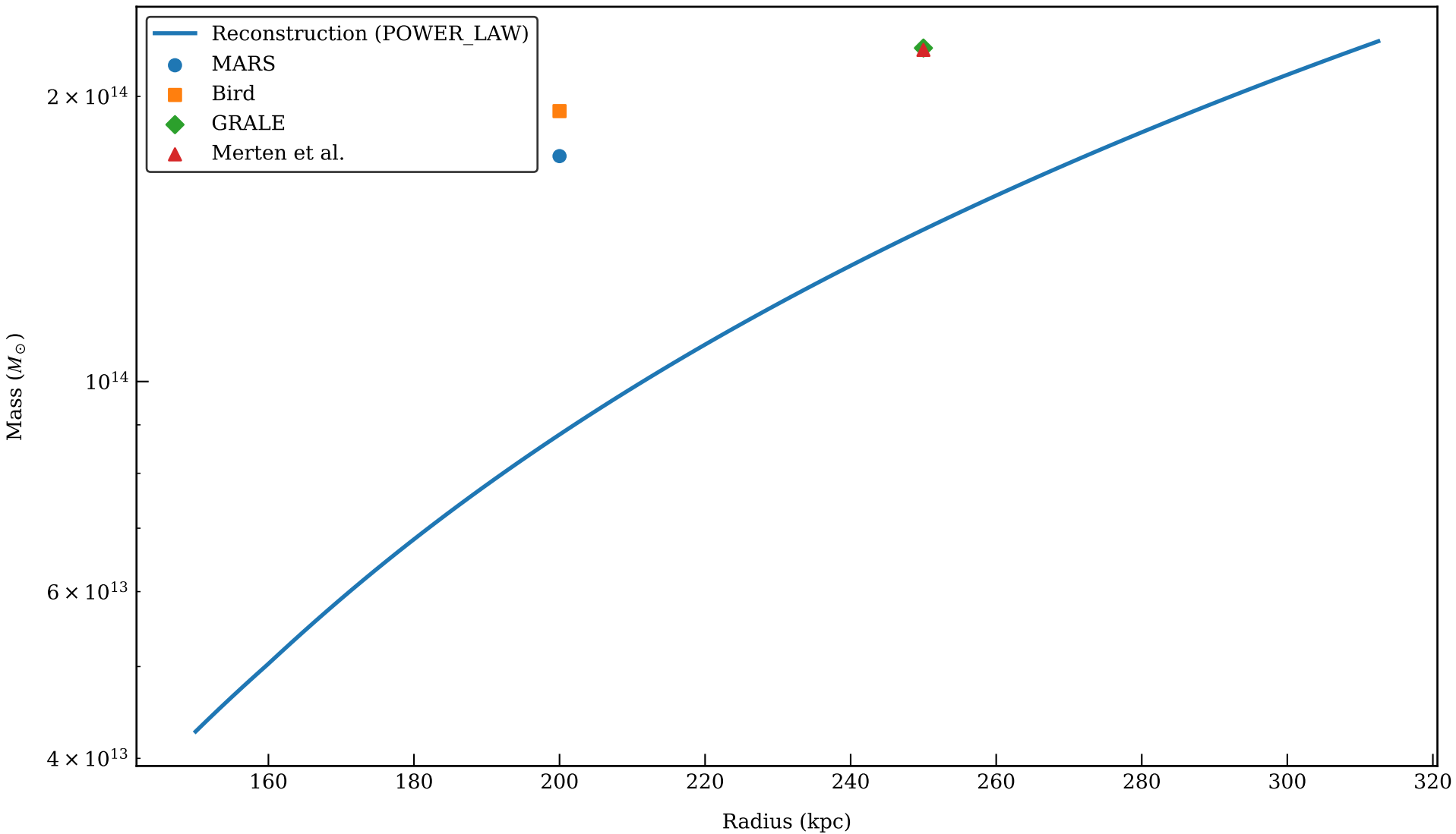
Mass Comparison: ABELL_2744 (POWER_LAW, WL+SL, signals: shear_f)
