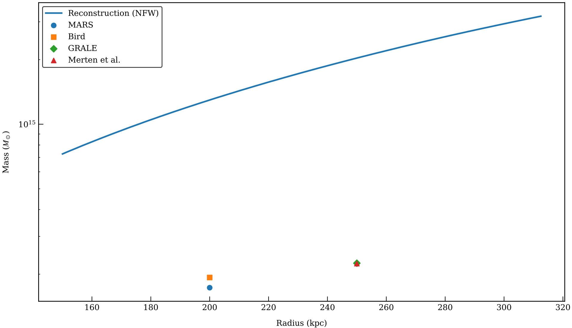
Mass Comparison: ABELL_2744 (NFW, WL+SL, signals: shear_g)
