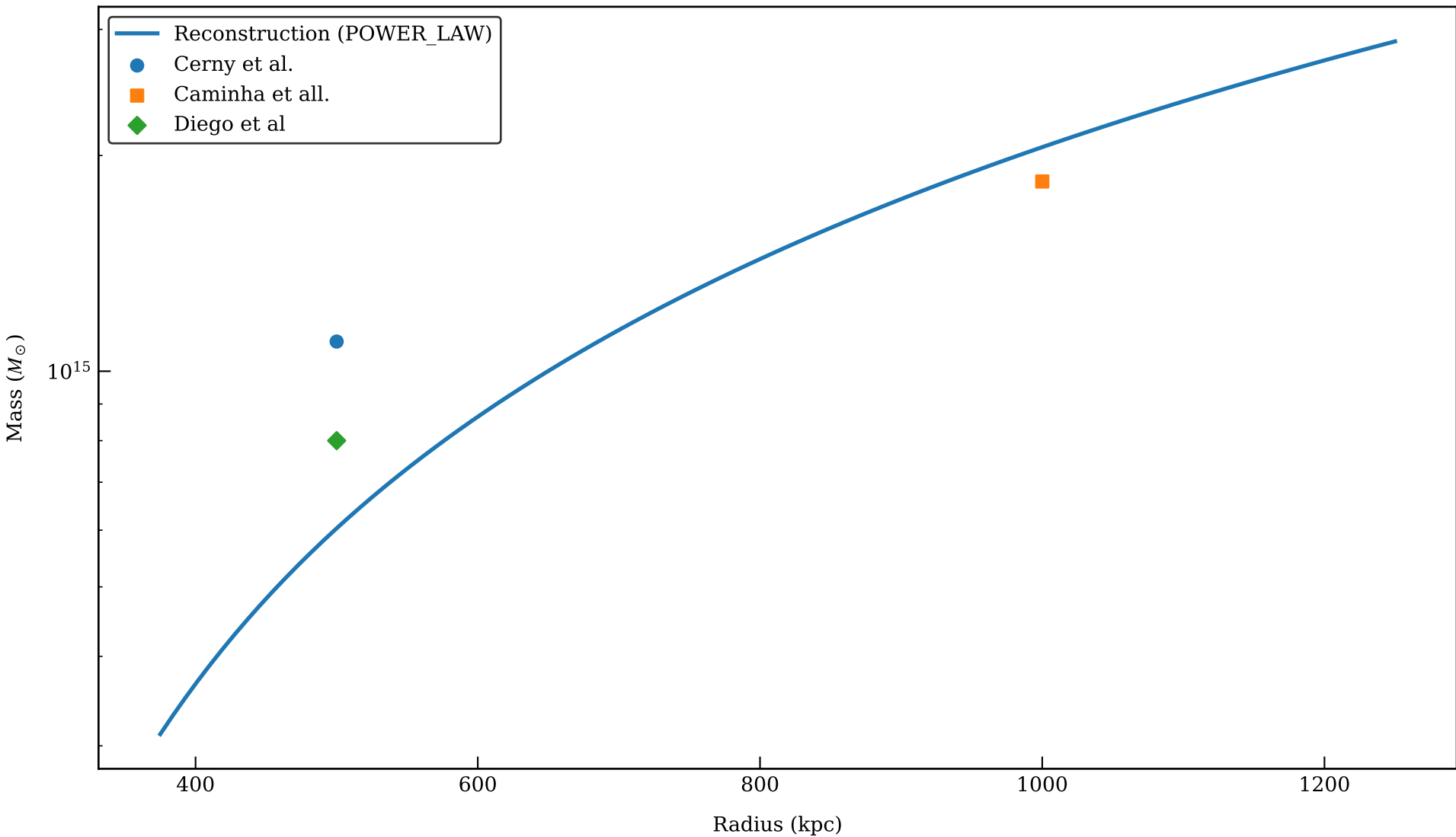
Mass Comparison: EL_GORDO (POWER_LAW, signals: f_g)
