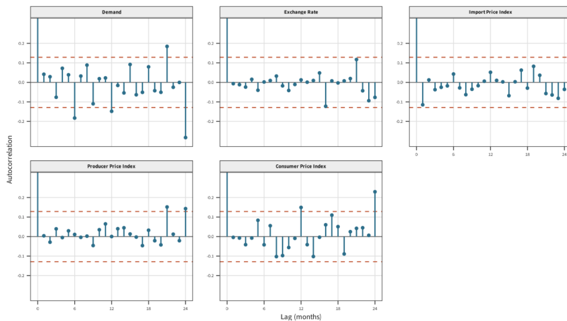
Figure 18: Autocorrelation Functions 1990 - 2010
