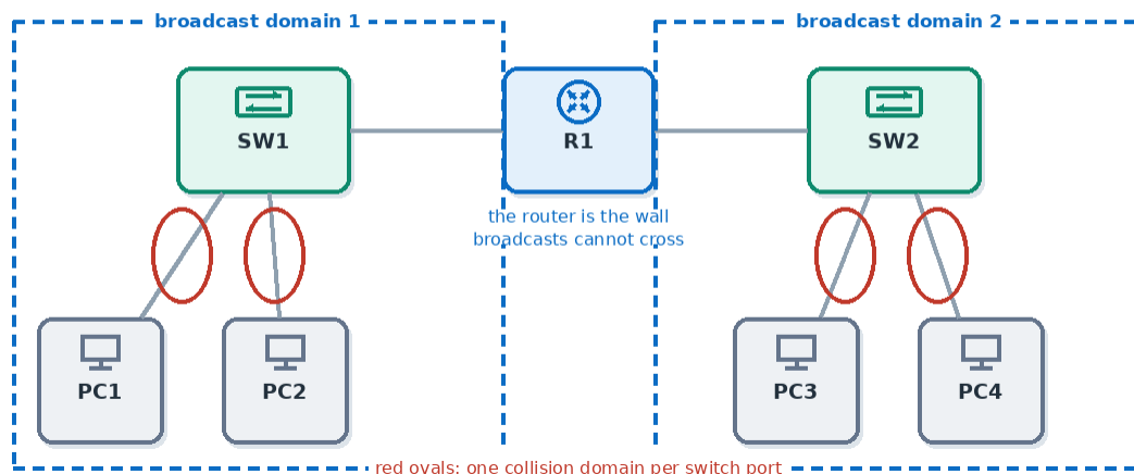
Collision domains (per port) vs broadcast domains (per VLAN / router side)
