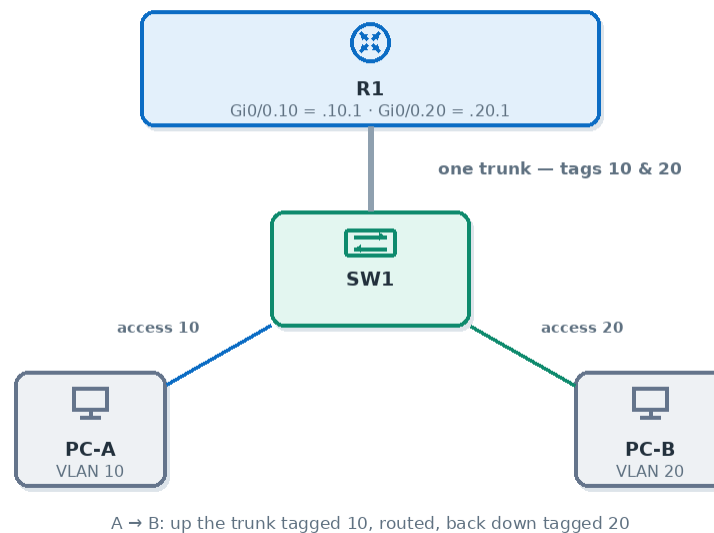
Router-on-a-stick — one trunk, one subinterface per VLAN
