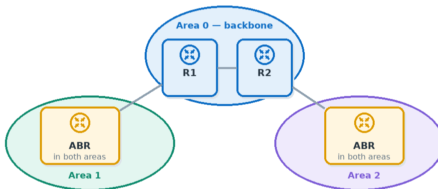
OSPF areas — every area touches the backbone
