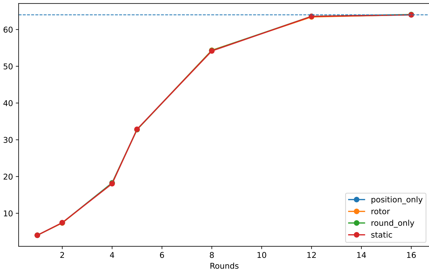
Mean plaintext-avalanche distance (bits)
