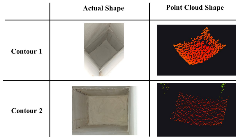
Figure 4.15. Actual and Point Cloud Surface Contour of Test 1
