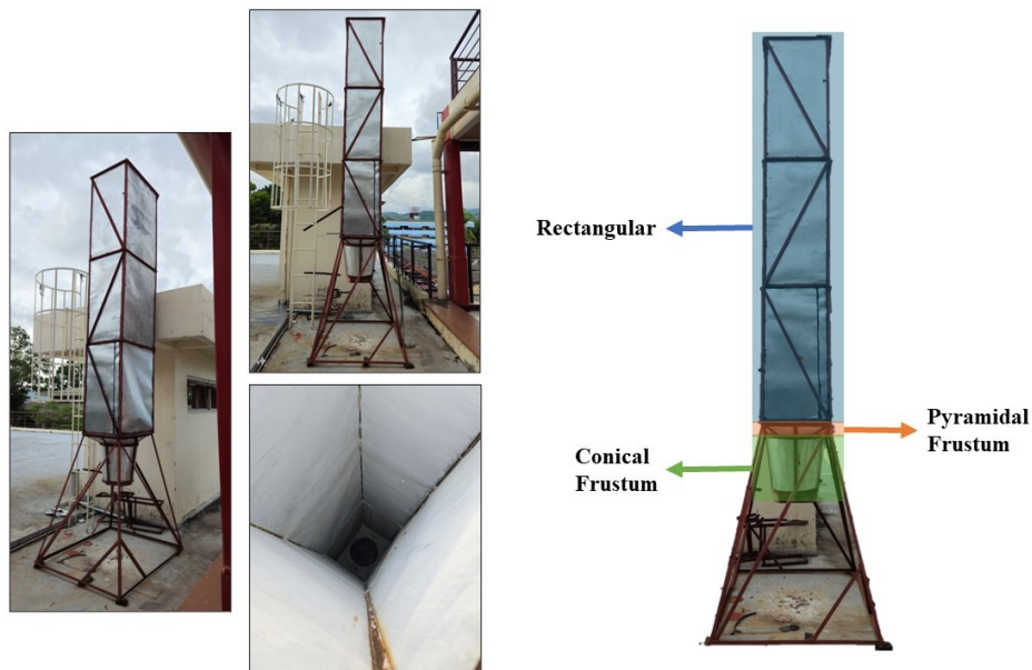
Figure 4.10. Actual Flour Storage Bin Created
