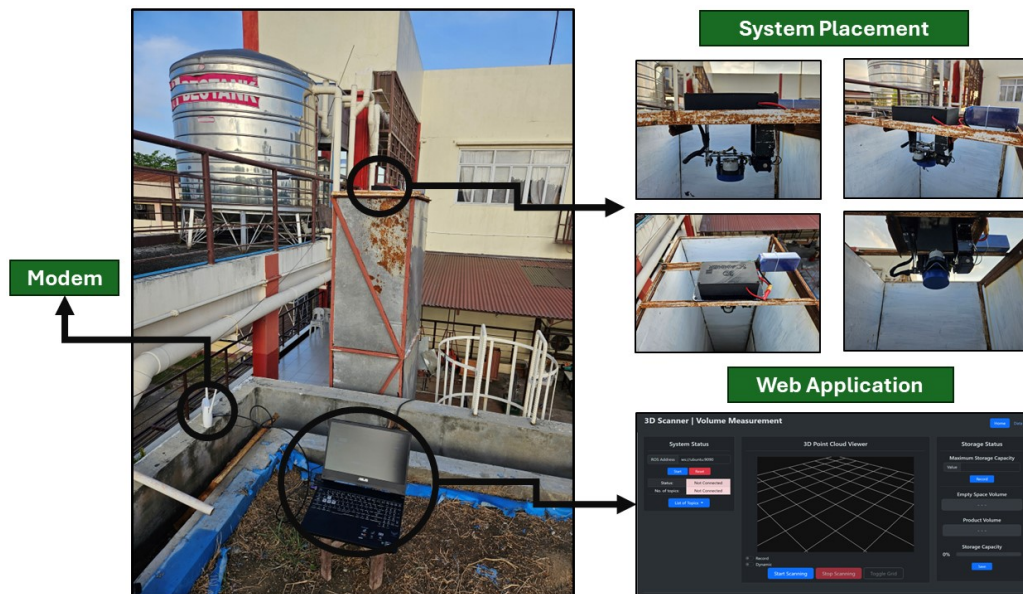
Figure 4.11. Testing Field and The Actual System Setup
