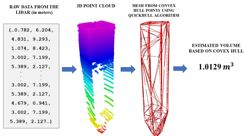
Figure 4.6. Example of the Volume Estimation Process of the System
