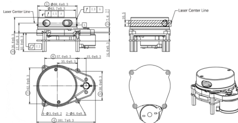
FIG 1 YDLIDAR X4 INSTALLATION AND MECHANICAL DIMENSIONS (UNIT:MM)
