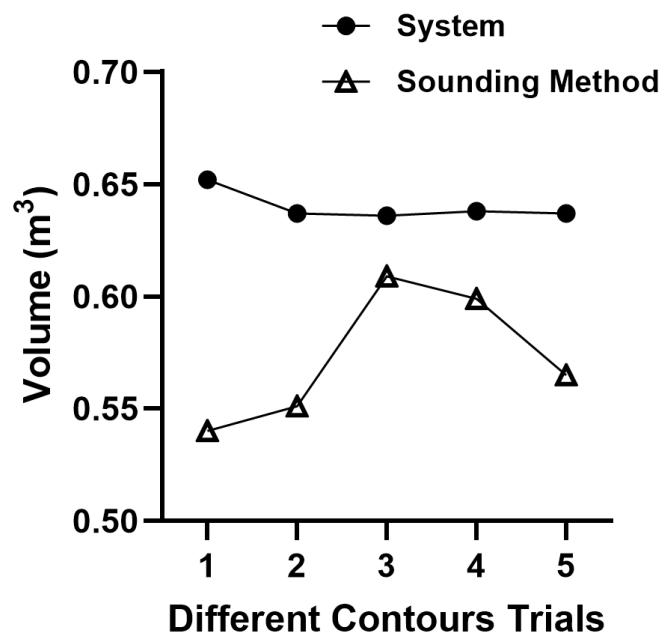
Figure 4.18. Distribution of volume measurements obtained from the system and sounding
