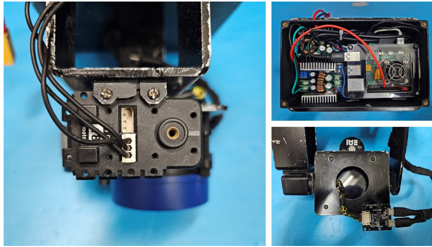
Figure 4.5. Actual Circuit Components of the System
