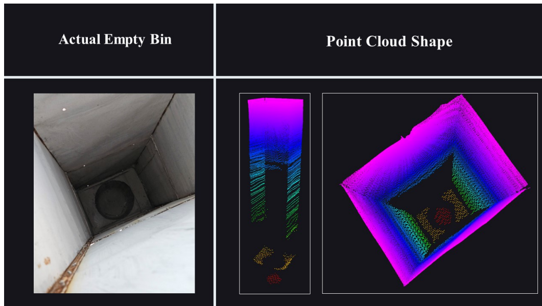
Figure 4.12. Actual Empty Bin and Scanned Point Cloud Data
