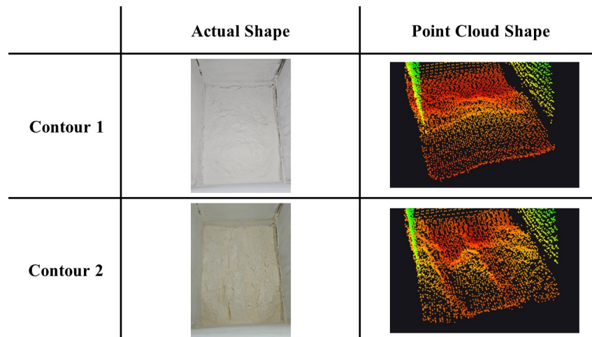
Figure 4.17. Actual and Point Cloud Surface Contour of Test 3
