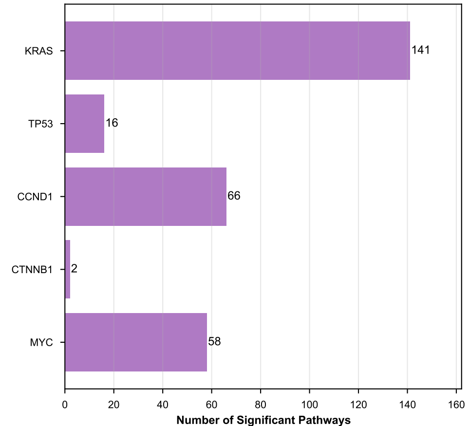
C) Pathway Enrichment (FDR<0.05)
