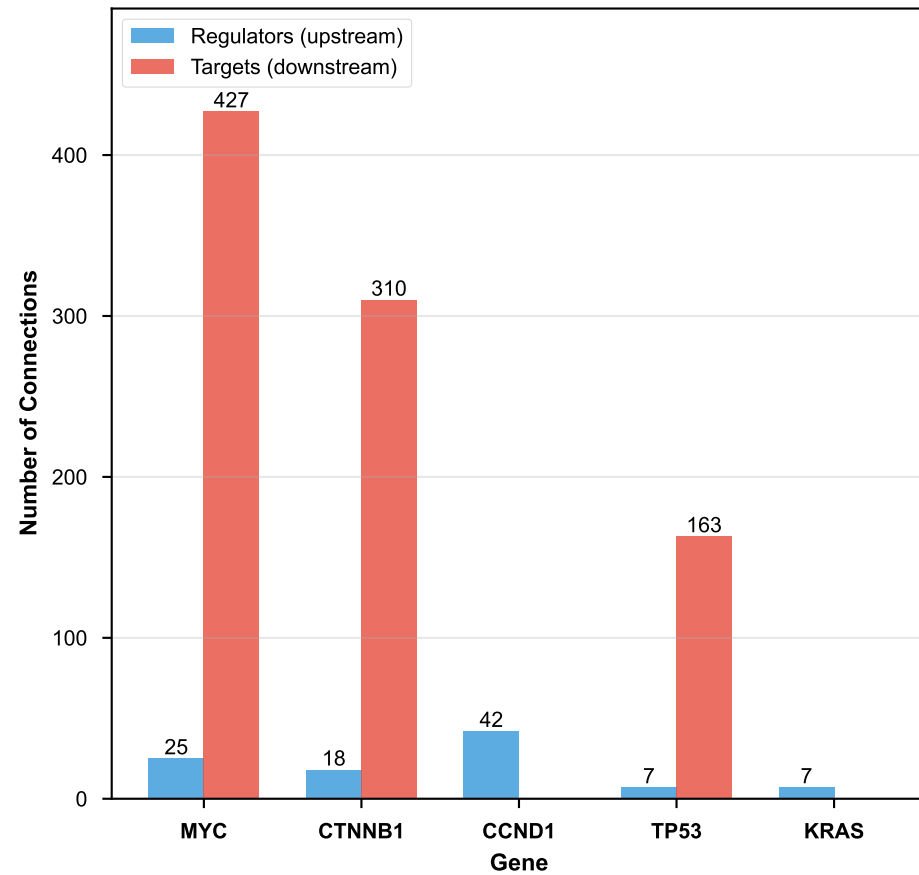
A) Regulatory Network Architecture
