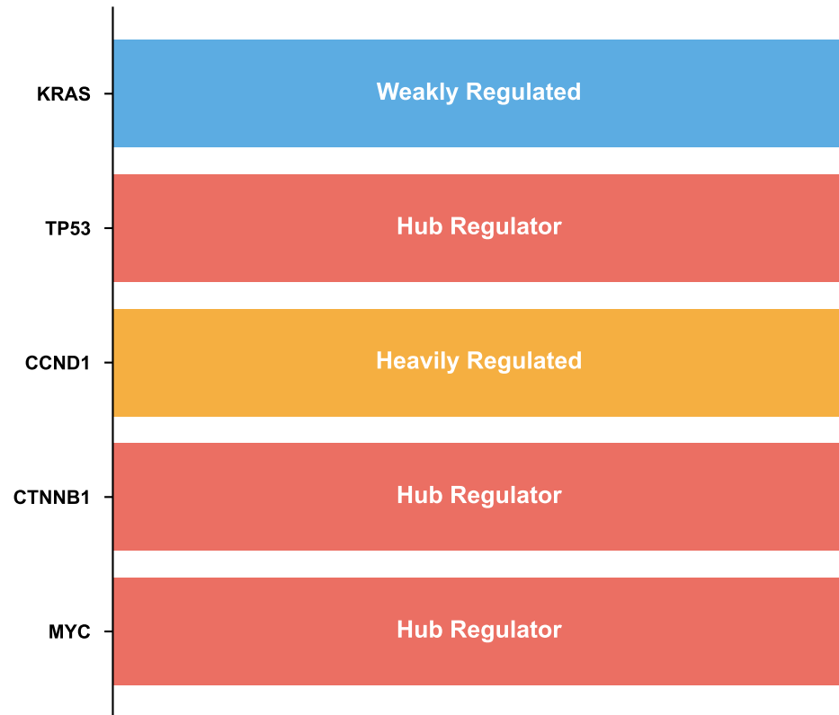
B) Network Regulatory Role
