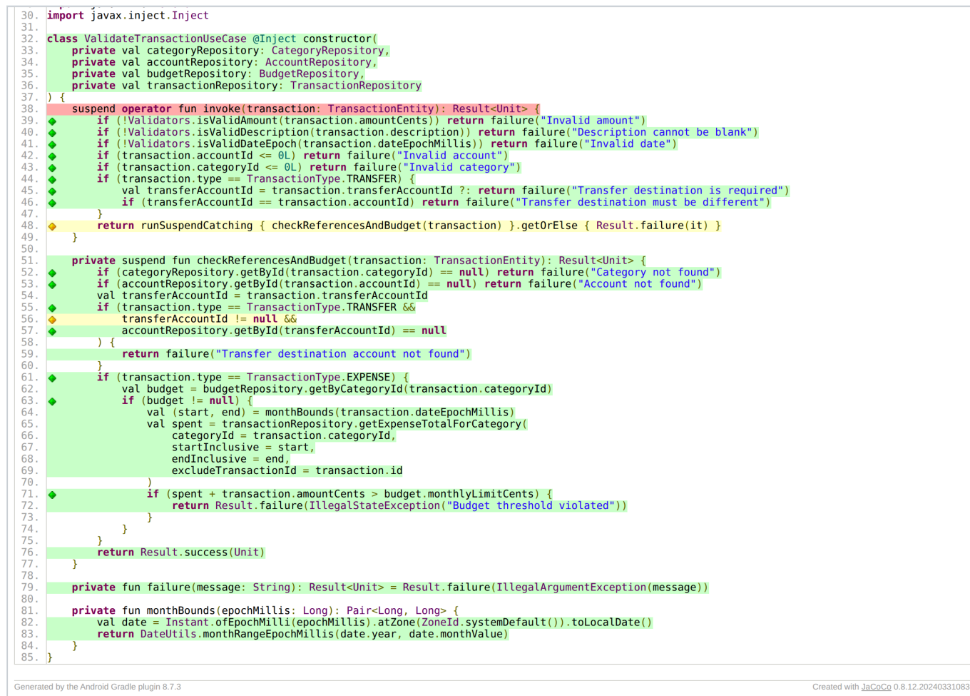
Figure 6. Line-by-line coverage of ValidateTransactionUseCase.kt . Green means executed and a green diamond means all branches taken; yellow means some branches missed and red means not executed. Every return failure(...) line from the plan's decision flow is green.
