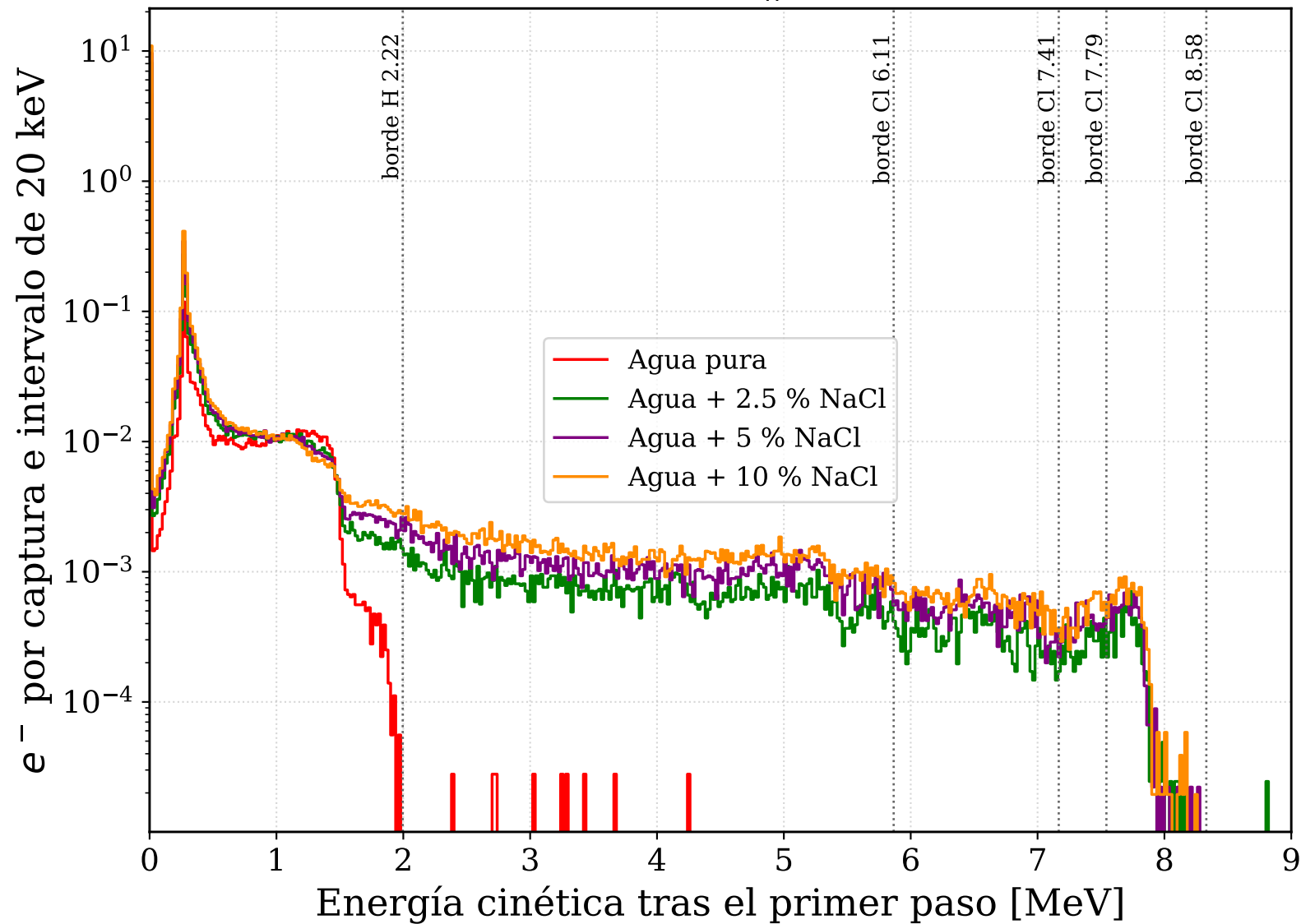
Electrones, E_n = 1 eV
