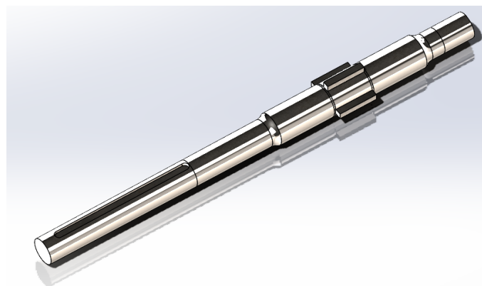
Figure 36: Optimal shaft design simulation tested with pinion load.
