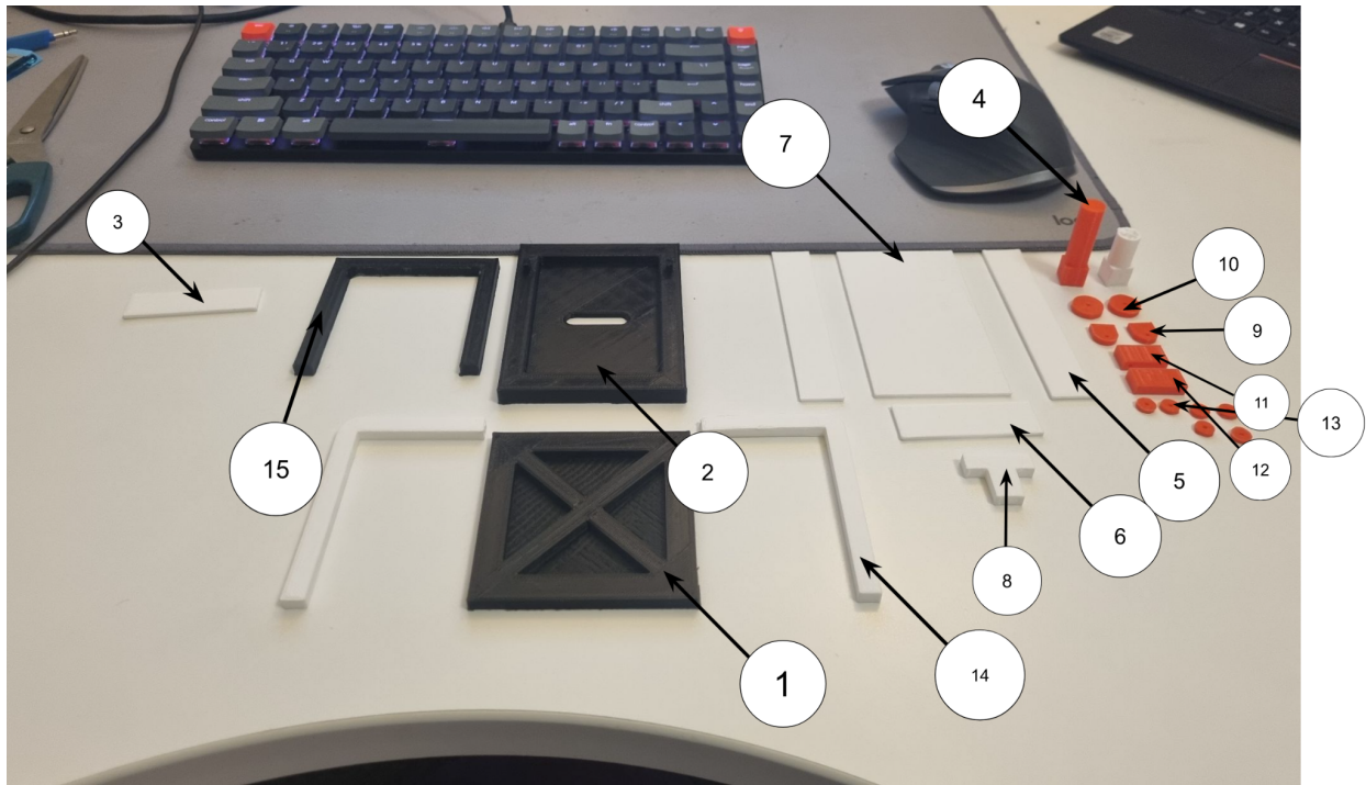
Figure 55: Parts for 3D assembly
