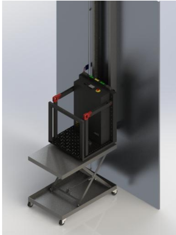
Figure 4: Final Design
