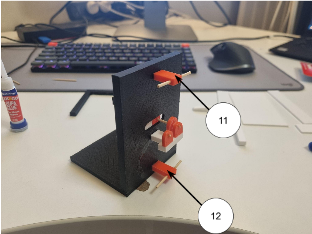
Figure 64: Assembly Step 9
