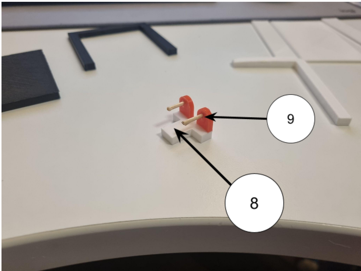
Figure 62: Assembly Step 7
