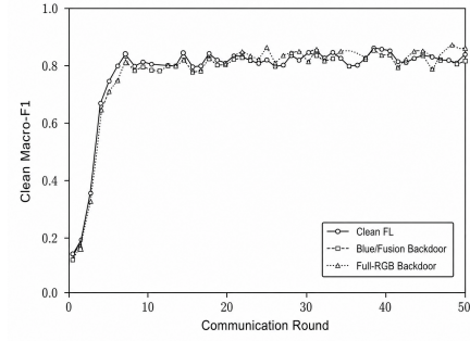
Fig. 5. Clean macro-F1 over FL communication rounds for the clean FL baseline and the strongest backdoor settings.
