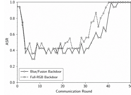
Fig. 6. Attack success rate (ASR) over FL communication rounds for the strongest blue/fusion and full-RGB backdoor settings.
