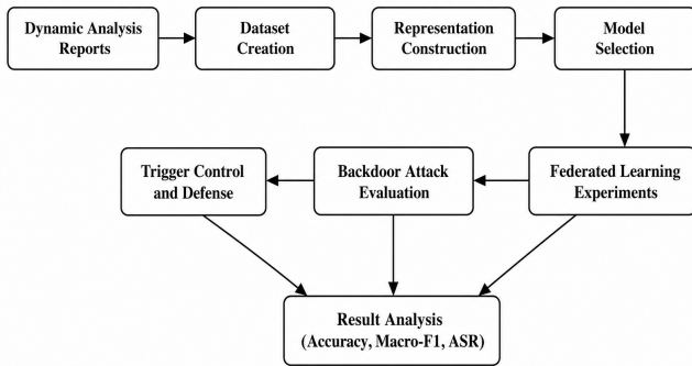
Fig. 1. Overall research workflow of the proposed study.
