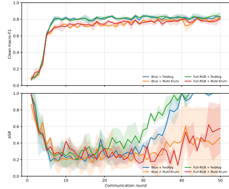
Fig. 7. Per-round clean macro-F1 and ASR across three random seeds for the blue/fusion and full-RGB backdoor settings under FedAvg and Multi-Krum. Shaded areas denote standard deviation across seeds.
