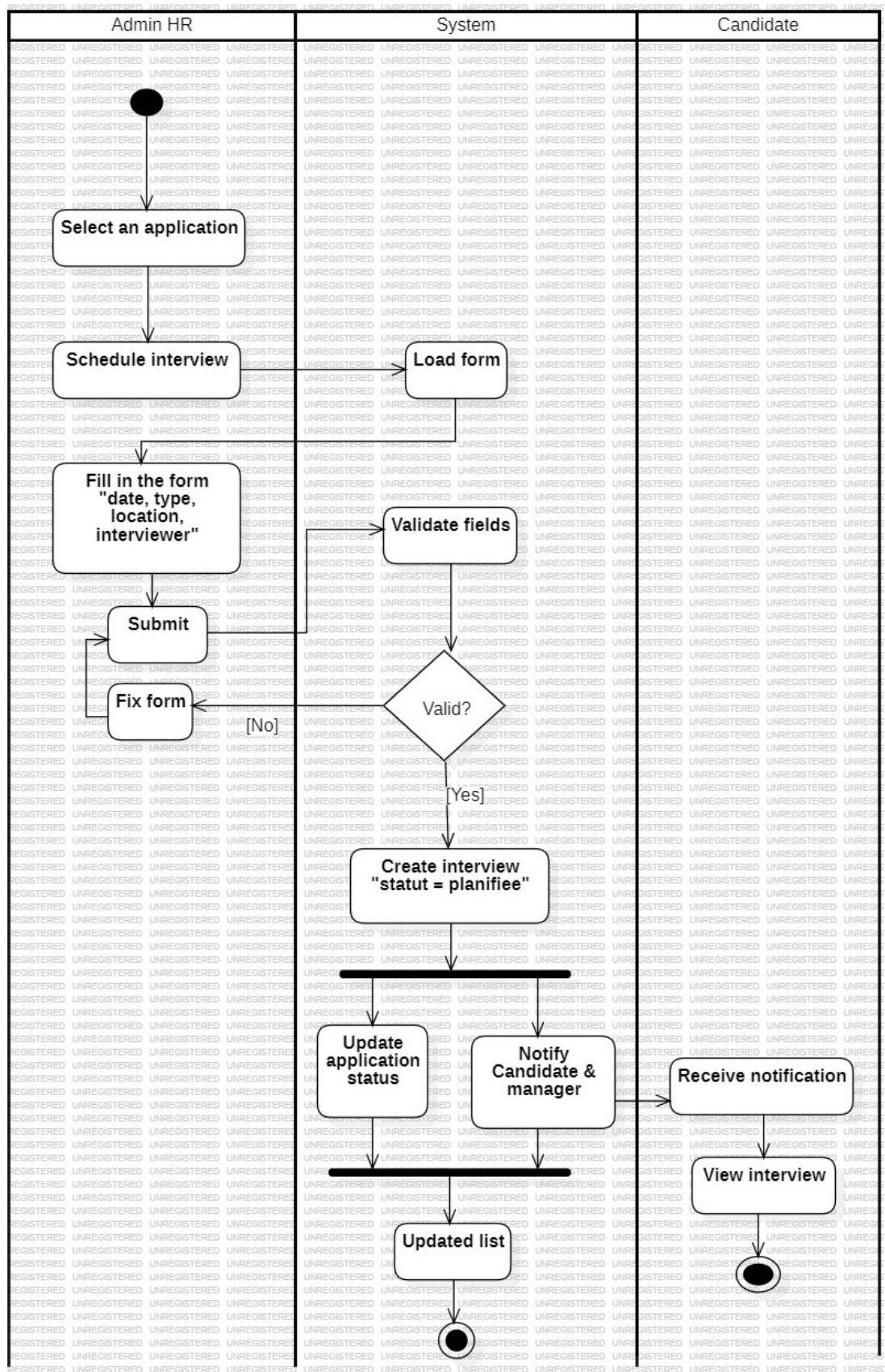
FIGURE 6.3 – Activity Diagram — Interview Planning
