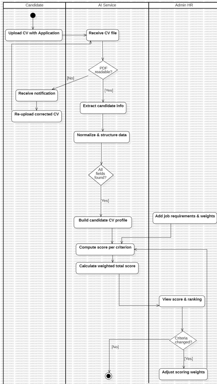
FIGURE 5.2 – Activity Diagram — CV Analysis and Scoring
