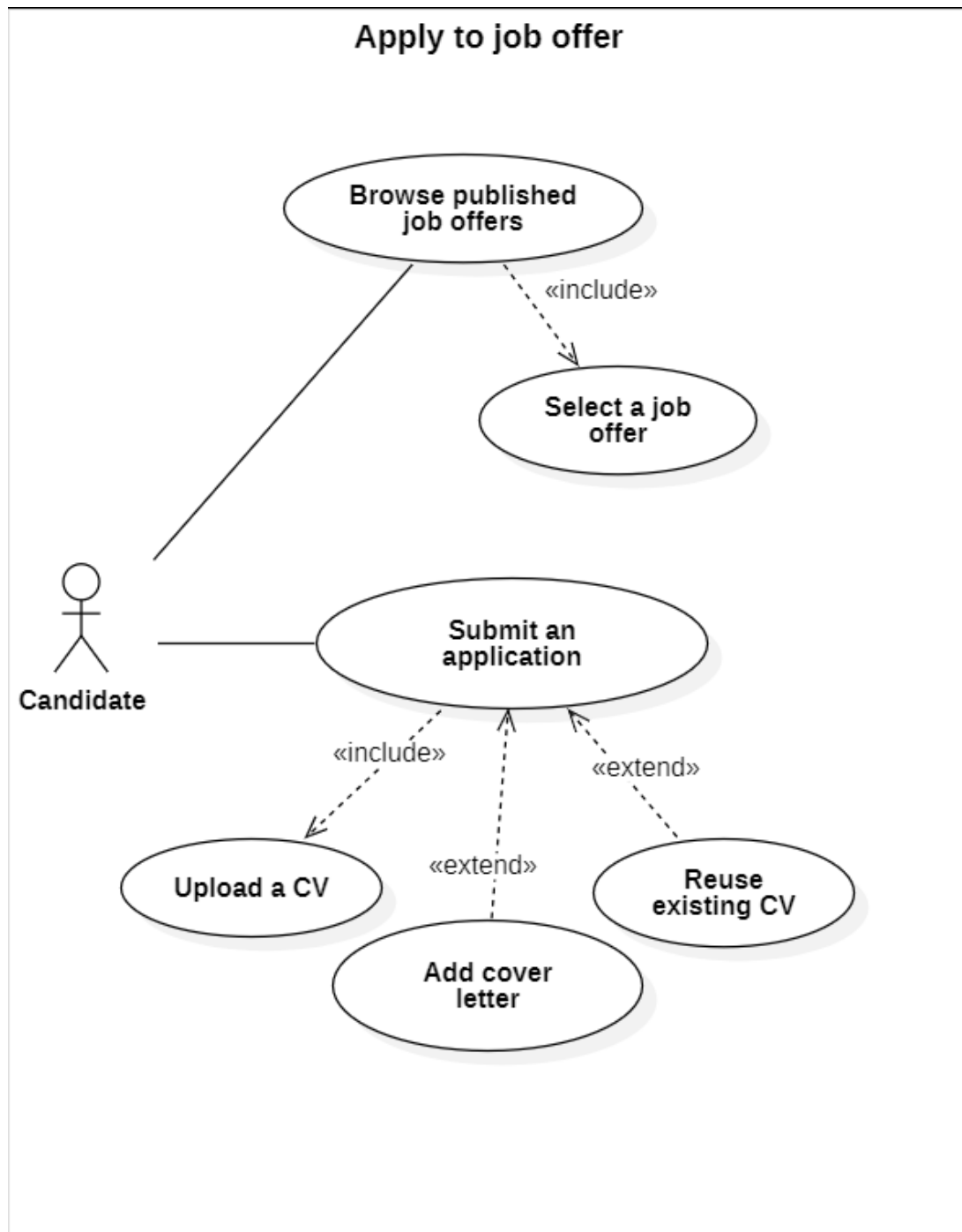
FIGURE 4.2 – use case Apply to a job offer— Sprint 2 : Recruitment Management
