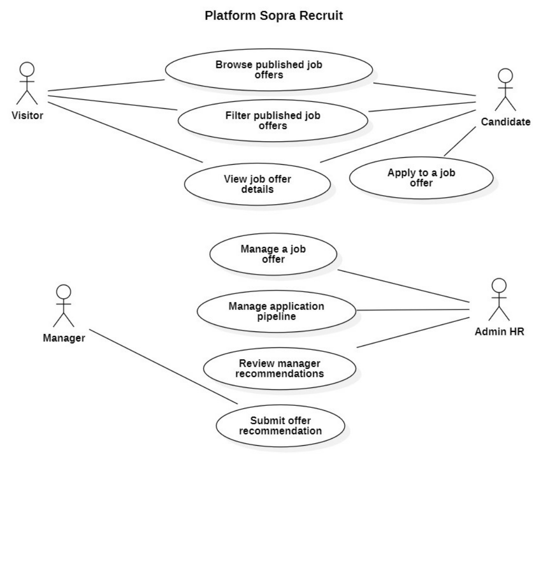
FIGURE 4.1 – Use Case Diagram — Sprint 2 : Recruitment Management
