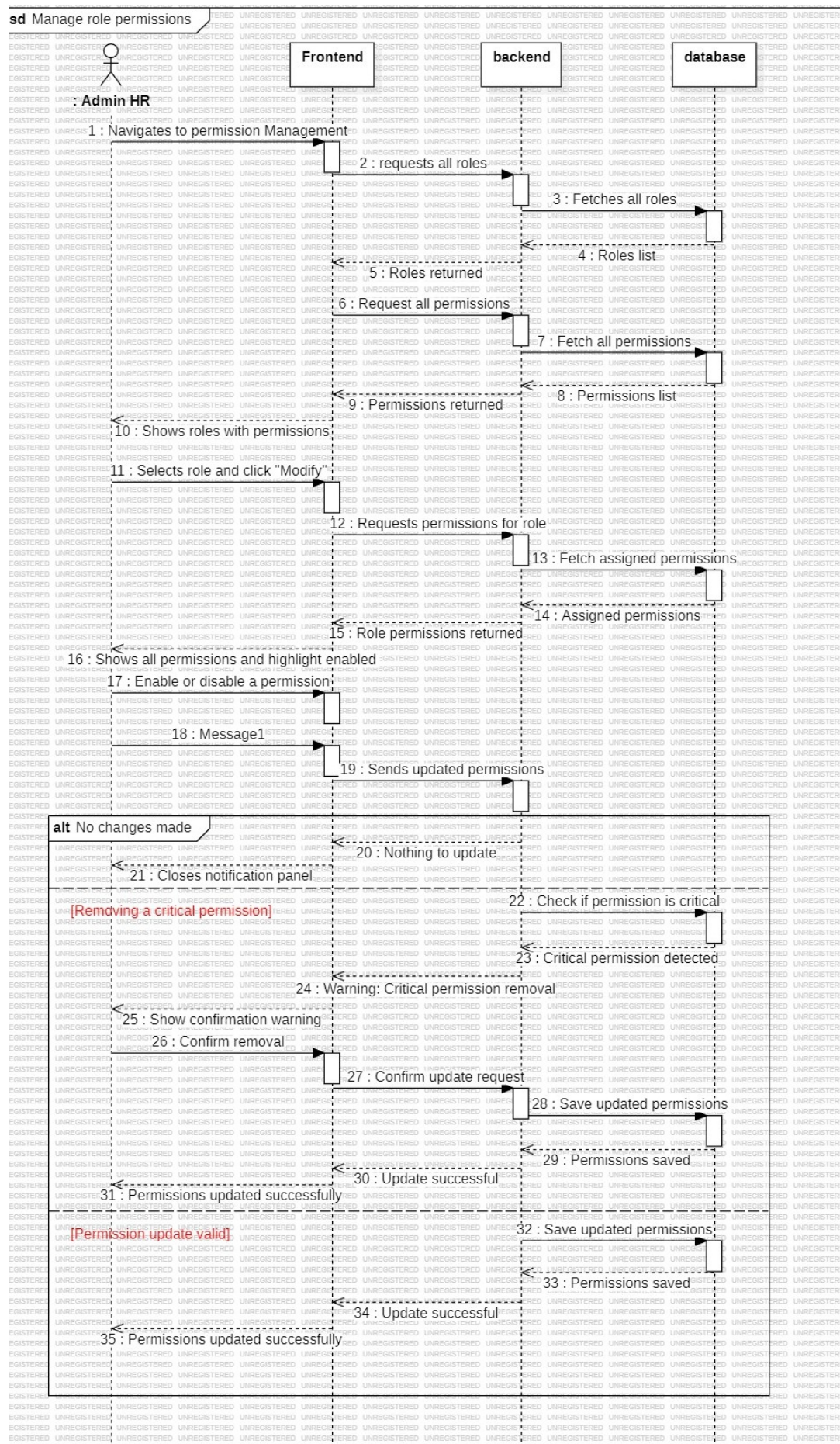
FIGURE 3.5 – Sequence Diagram — Manage Permission
