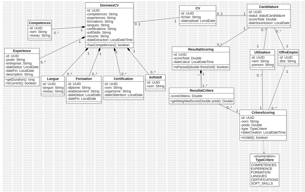
FIGURE 5.3 – Class Diagram — Sprint 3
