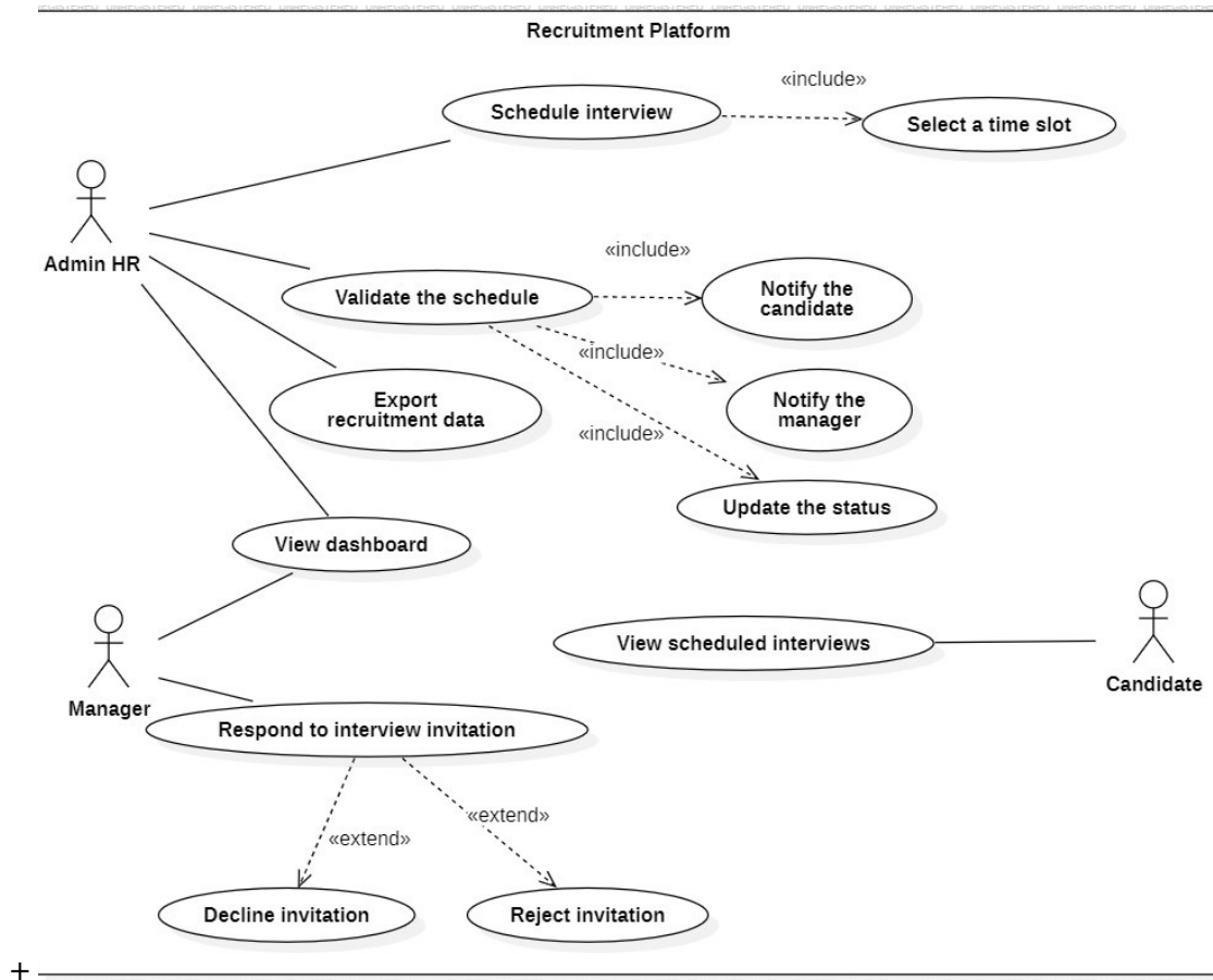
FIGURE 6.1 – Global Use Case Diagram — Final System
