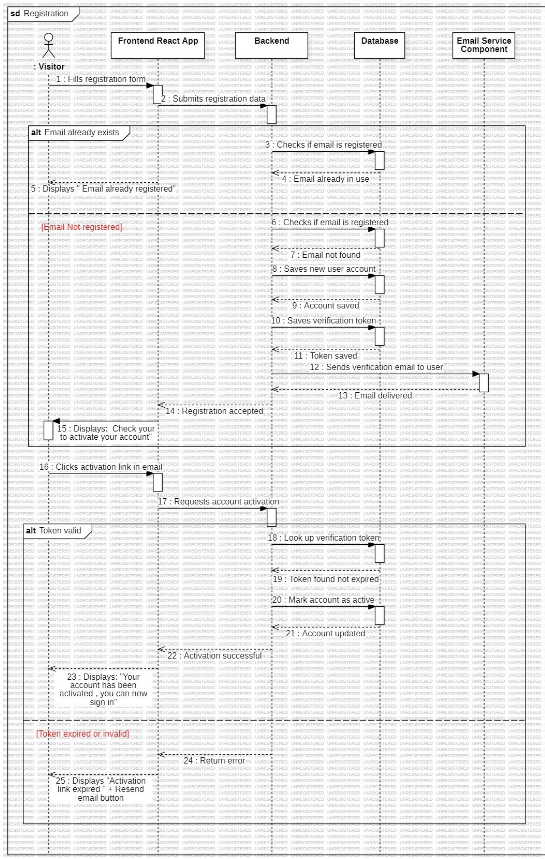
FIGURE 3.2 – Sequence Diagram — Register
