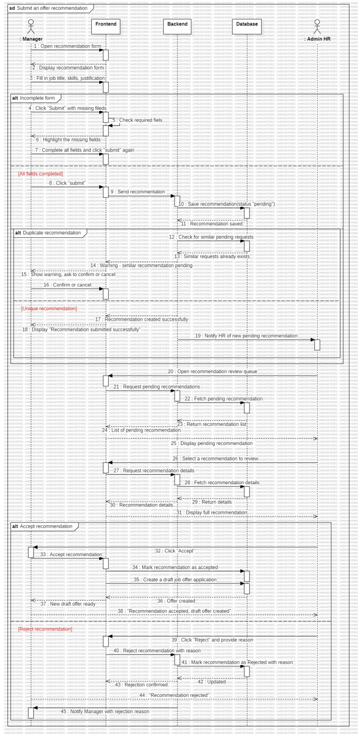
FIGURE 4.7 – Sequence Diagram — Submit Offer Recommendation
