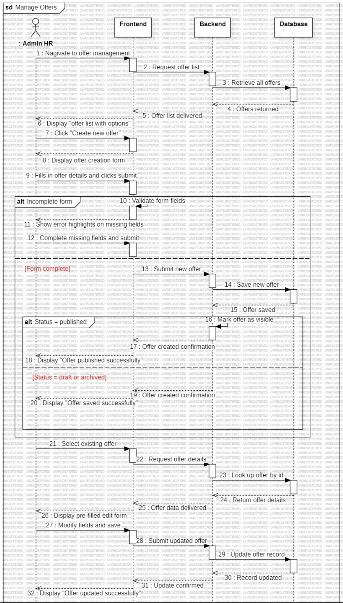
FIGURE 4.4 – Sequence Diagram — Manage Job Offer
