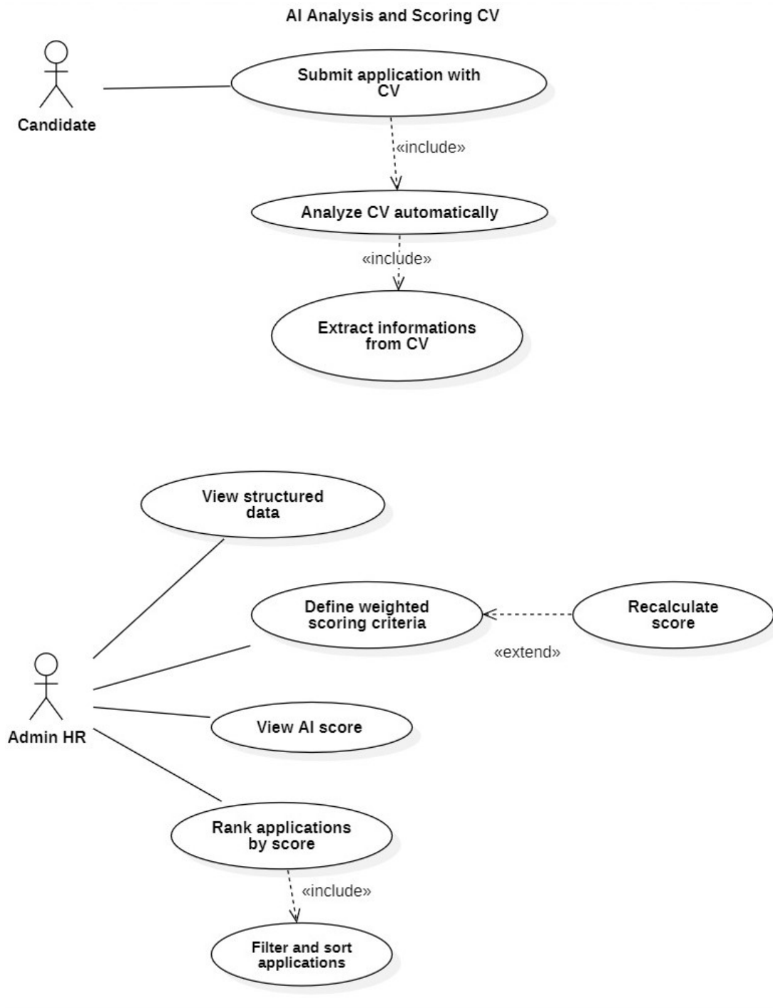
FIGURE 5.1 – Use Case Diagram — Sprint 3
