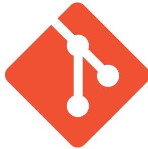
FIGURE 2.5 – Git Logo
