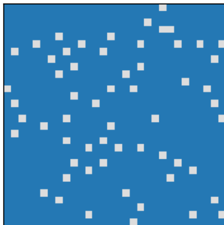
Cooperation first r=4.8; final C=0.934
