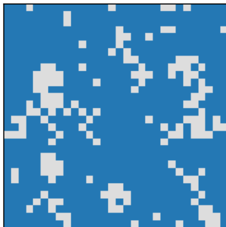
Upper-tail filter r=4.8; final C=0.830
