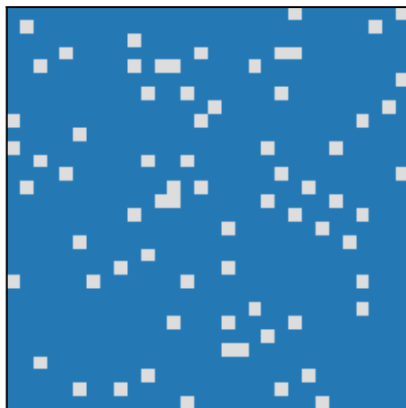
Learned controller r=4.8; final C=0.921
