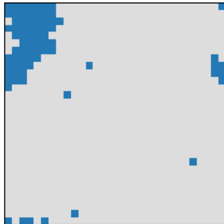
Global NI (k=0.5) r=4.8; final C=0.134
