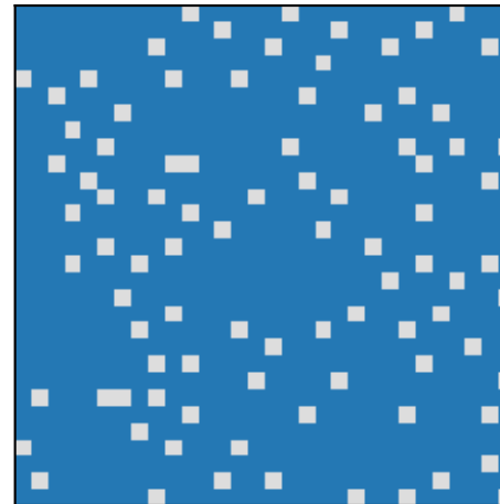
Cooperation first (k=0.5) r=4.8; final C=0.936
