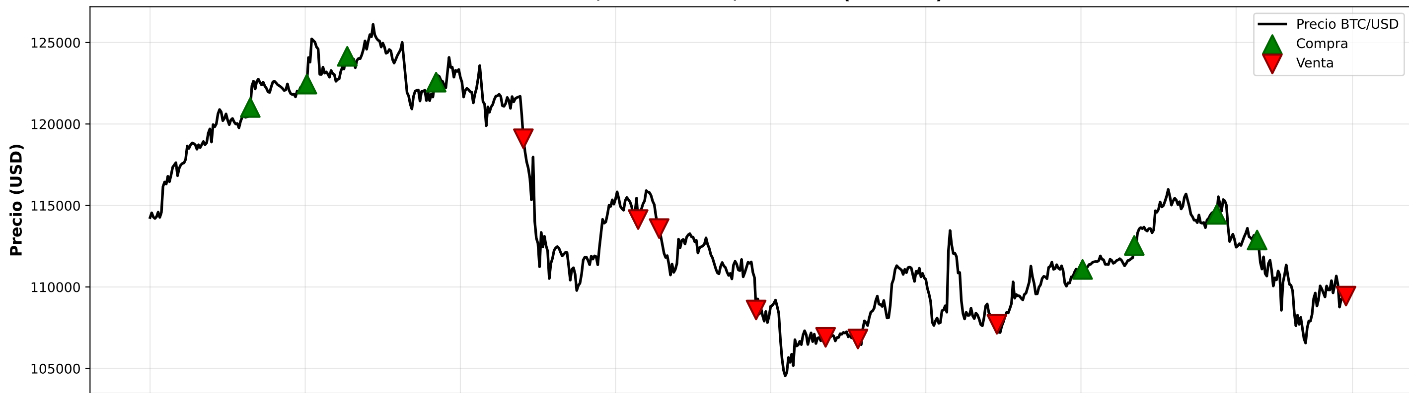
BTC/USD - SMA 7/20 Mixed (2025-10)
