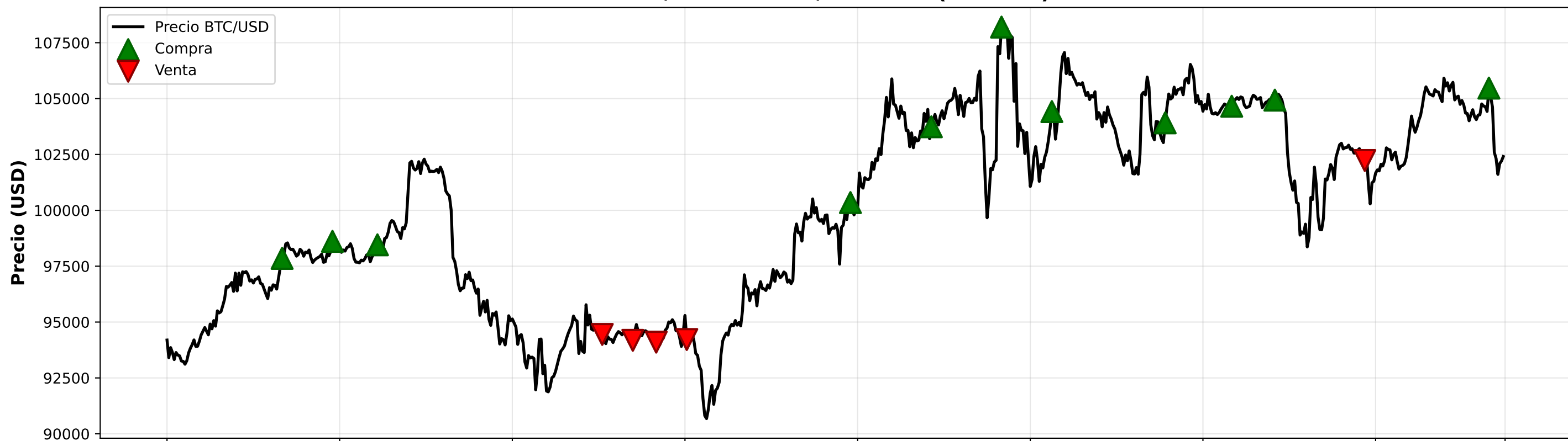
BTC/USD - SMA 7/20 Mixed (2025-01)
