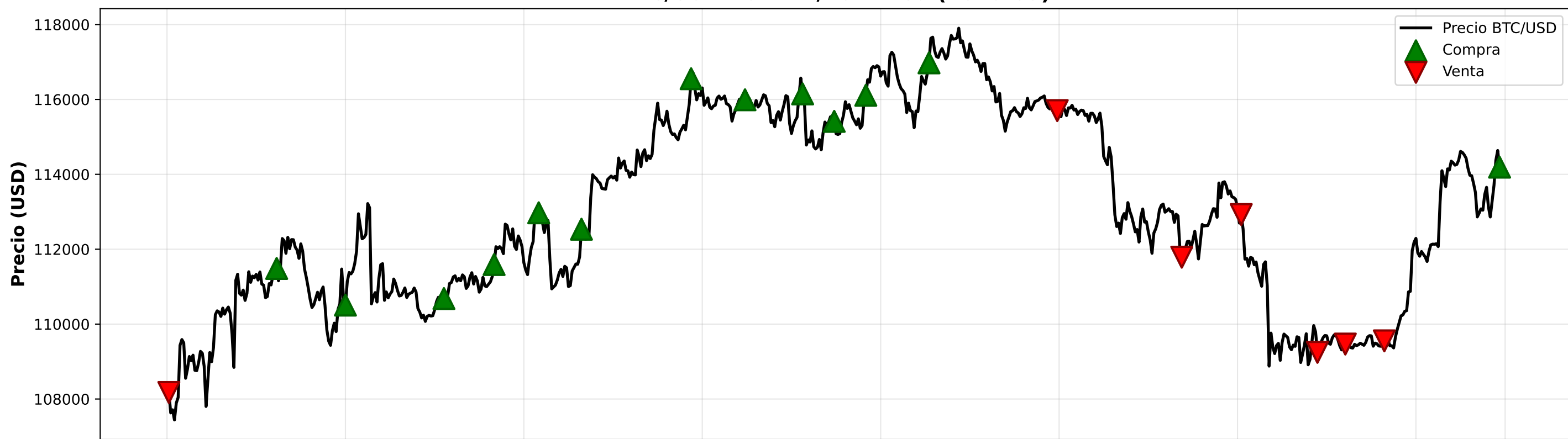
BTC/USD - SMA 7/20 Mixed (2025-09)
