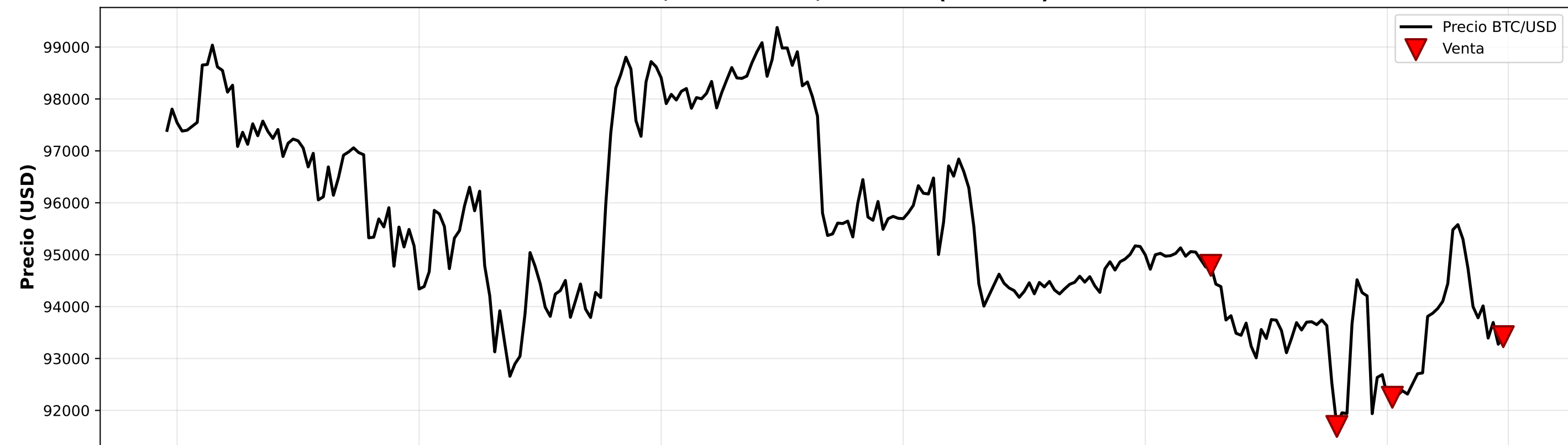
BTC/USD - SMA 7/20 Mixed (2024-12)
