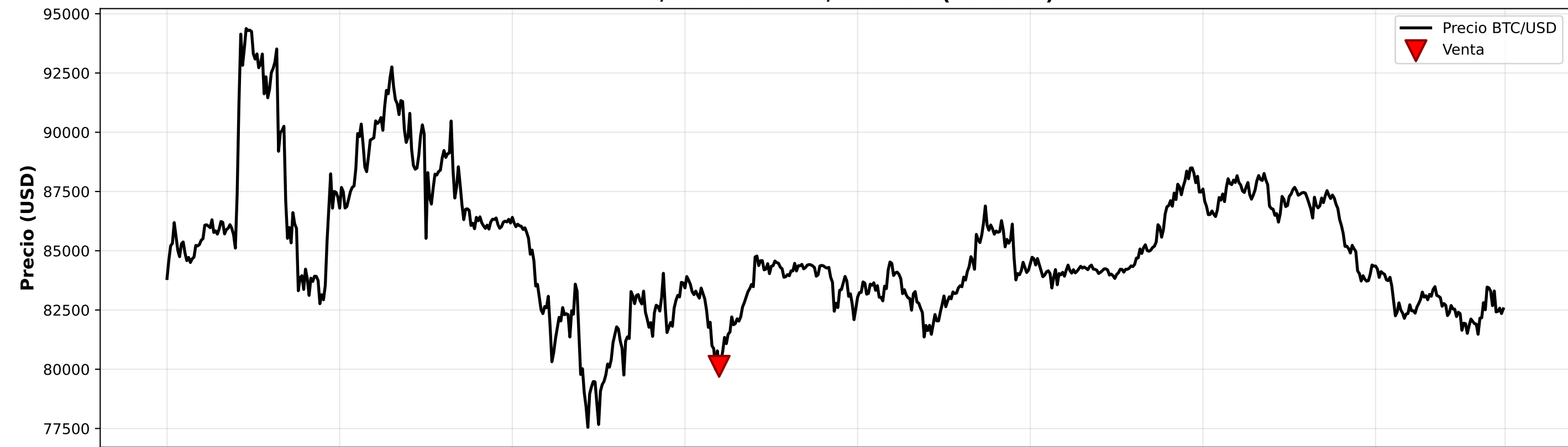
BTC/USD - SMA 20/50 Short (2025-03)
