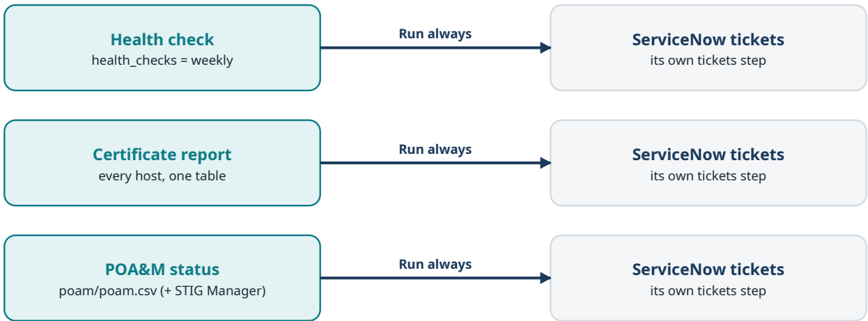
Weekly compliance: three independent chains, each with its own tickets step (a step with two parents would get only one parent's findings).
