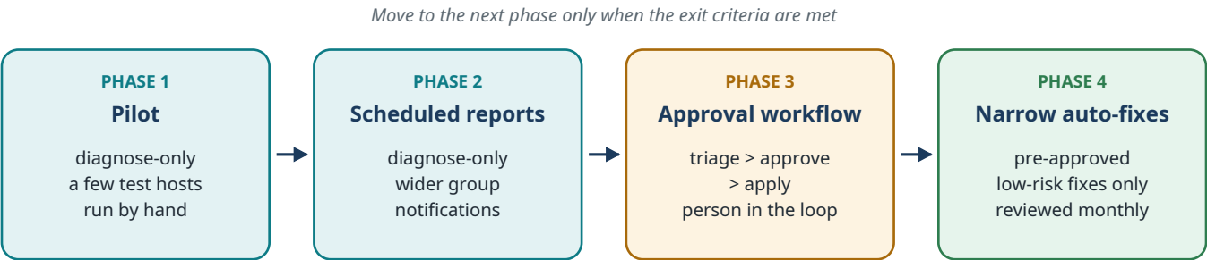
Figure 5. Rollout phases
