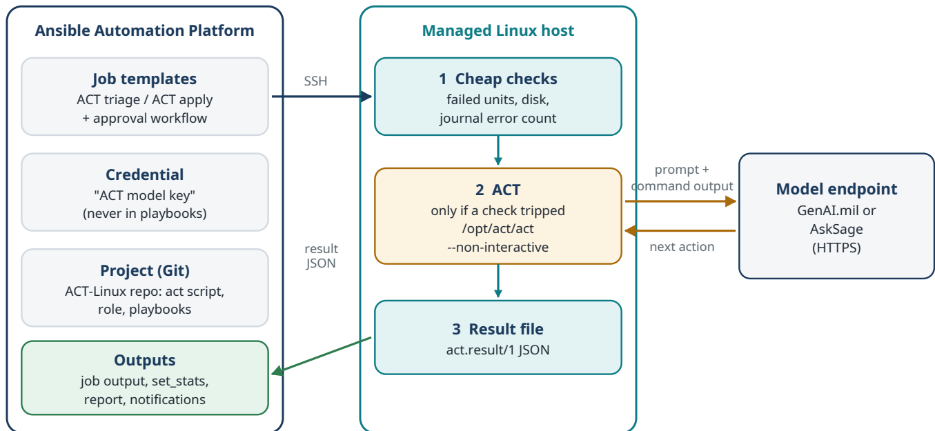
Figure 3. Components and data flow for one triage job
