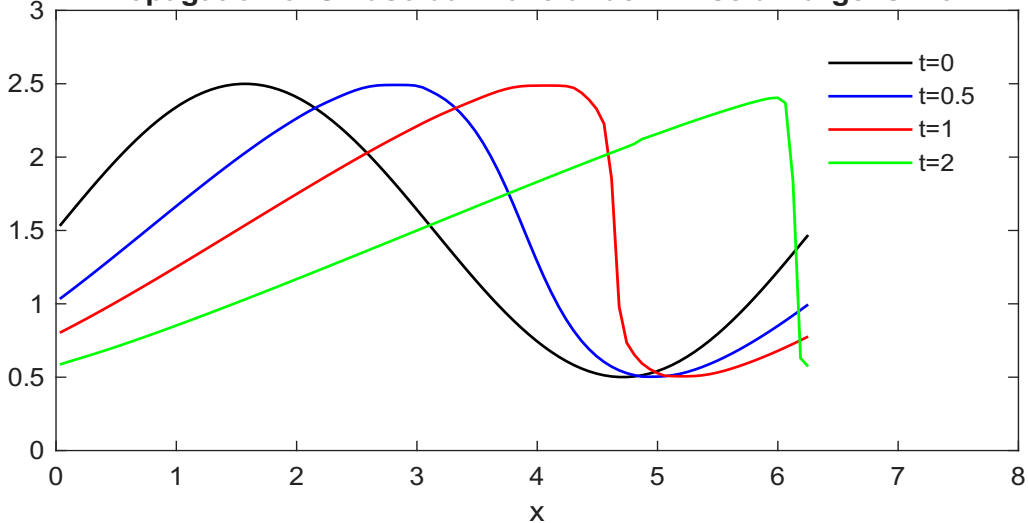
Propagation of Sinusoidal Wave under inviscid Burger's Flow
