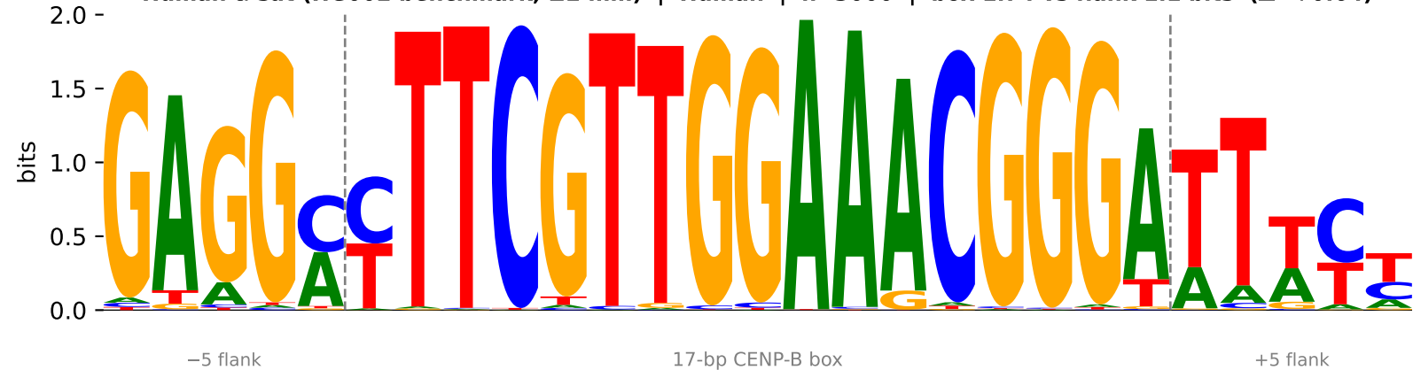
Human \alpha -sat (HG002 benchmark, \leq 2 mm) | Human | n=3000 | box 1.74 vs flank 1.1 bits ( \Delta=+0.64 )
