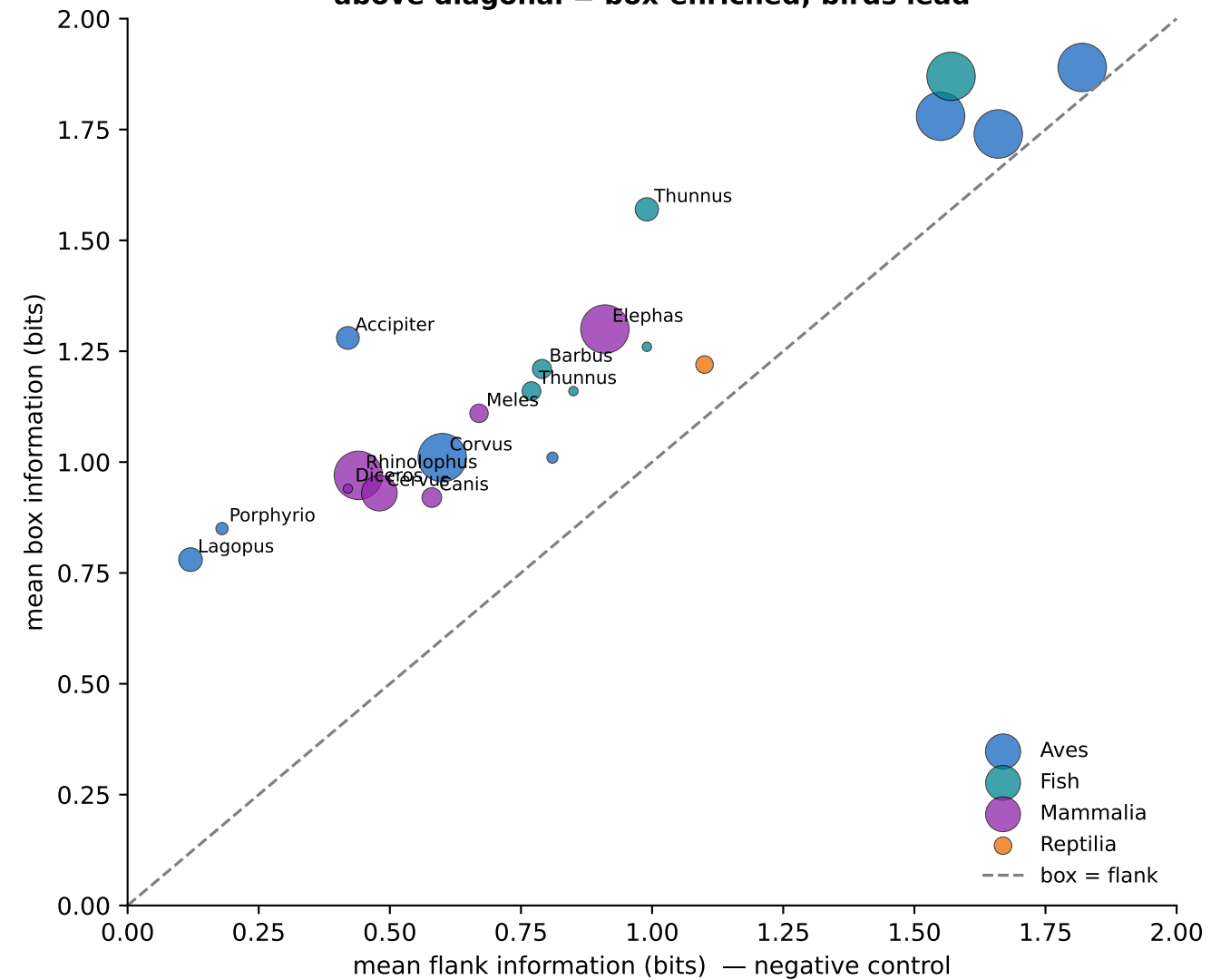
Vertebrates by subgroup (size \propto boxes/Mbp) above diagonal = box-enriched; birds lead
