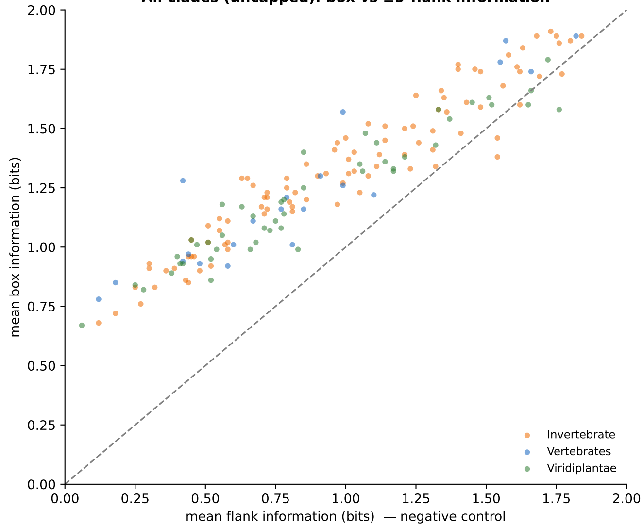
All clades (uncapped): box vs \pm 5 -flank information
