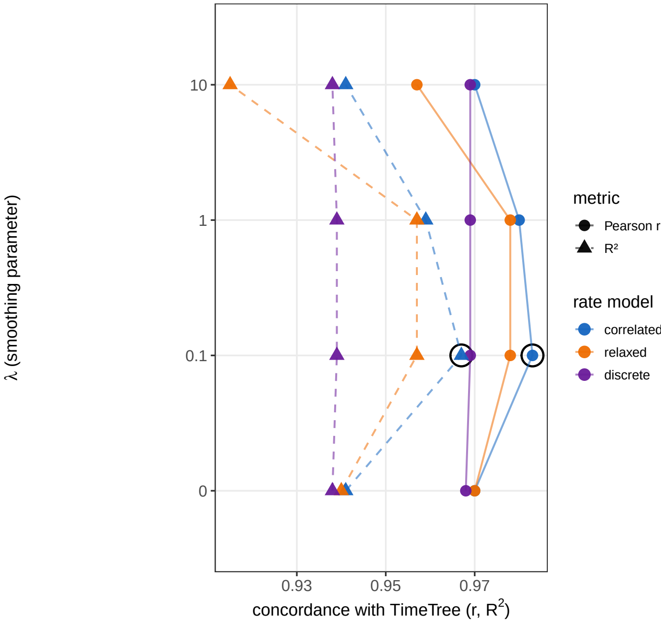
A: The 62 calibration nodes vs TimeTree (red diamond = TimeTree median; red line = TimeTree range / imposed constraint; black circle = calibrated age, chronos correlated). B: node-age concordance ( R^2 and Pearson r vs TimeTree; n = 213 nodes).
