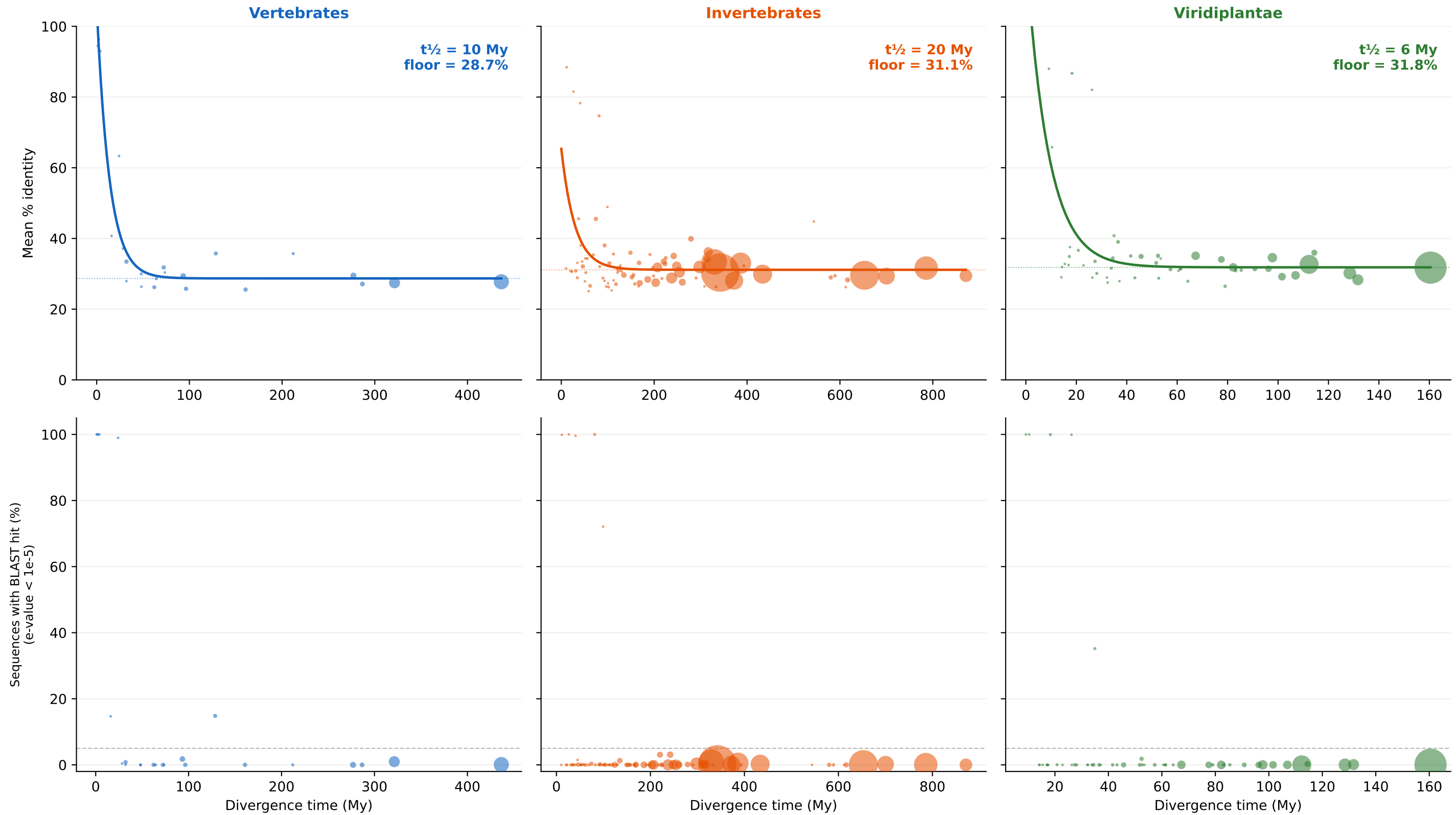
Satellite sequence similarity decay — BLASTN all-vs-all, node-averaged (325-sp) Top: mean % identity (C free — empirical floor). Bottom: detection rate (fraction with BLASTN hit, e < 1 \times 10^{-5} ).
