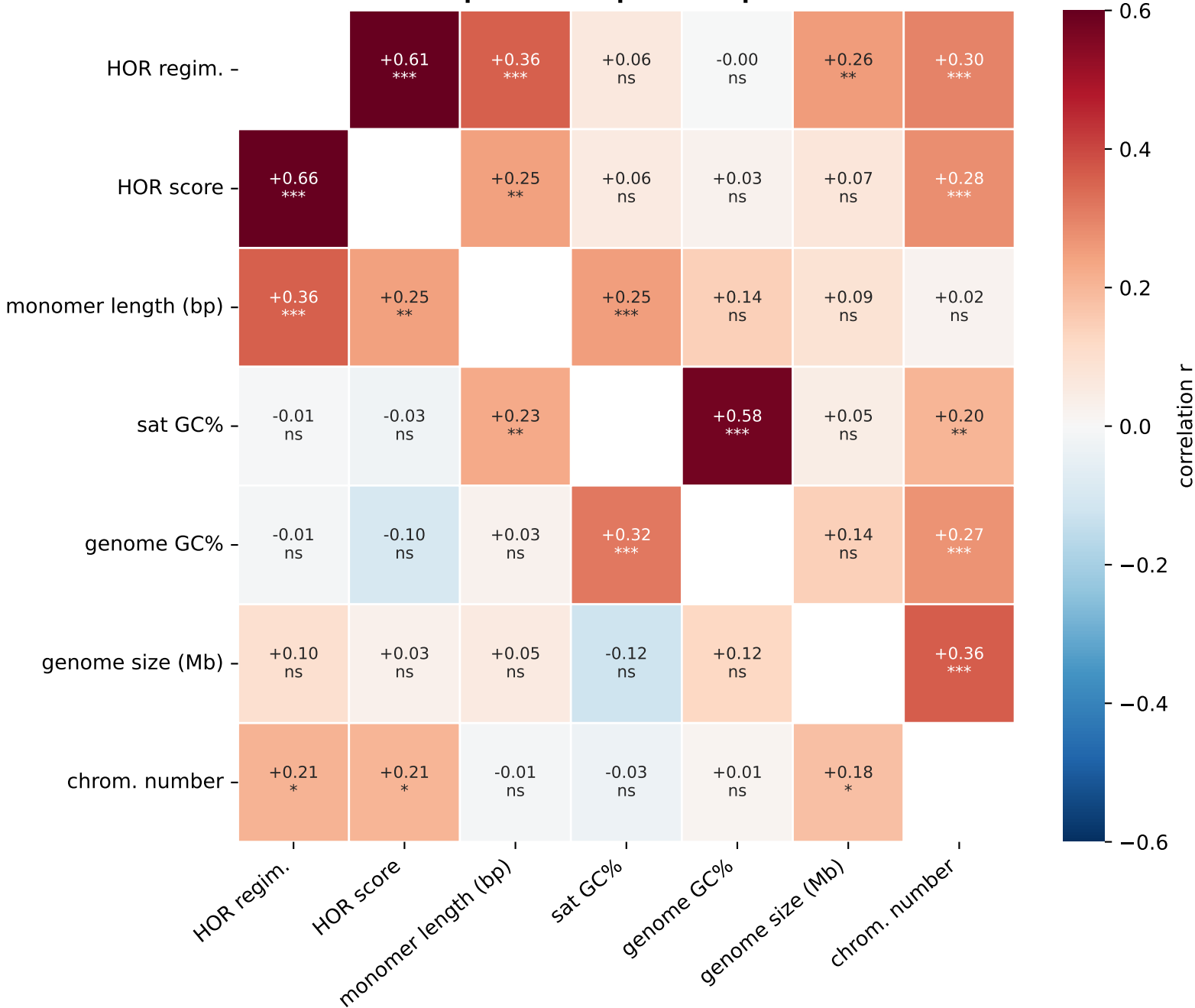
Trait correlations: upper = naive Pearson, lower = phylogenetic (PGLS, \lambda -adjusted) *** p<0.001 ** p<0.01 * p<0.05
