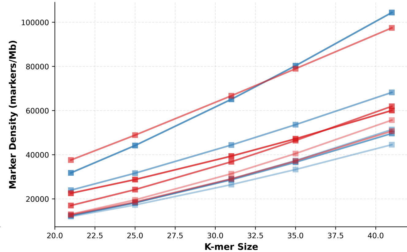
CEN Marker Density by Chromosome
