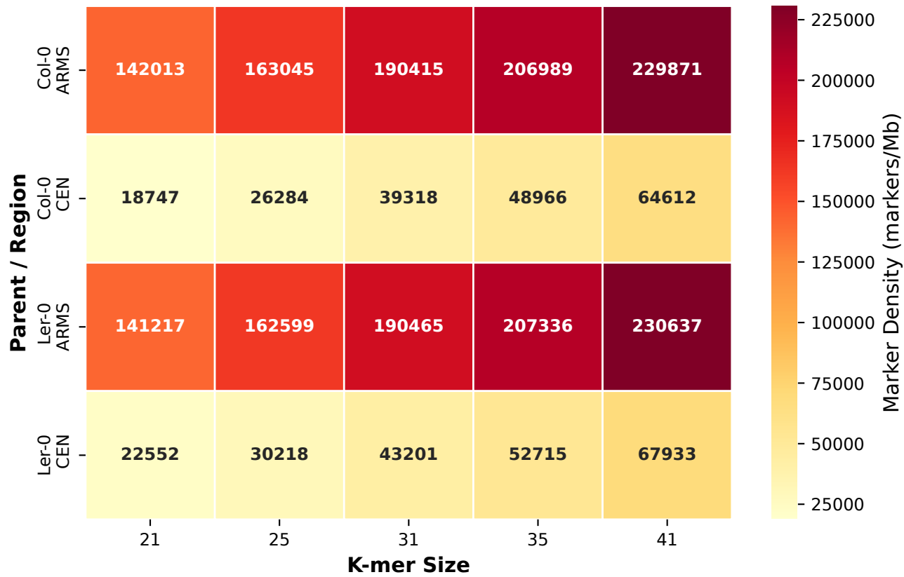
Marker Density Heatmap Across K-mer Sizes
