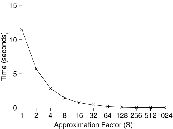
Figure 29.6: Scaling Approximate Counters
