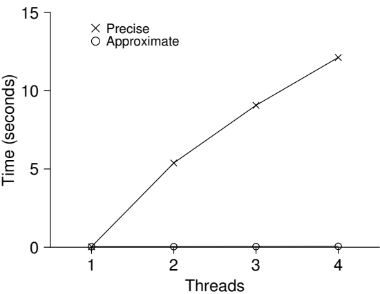
Figure 29.5: Performance of Traditional vs. Approximate Counters
