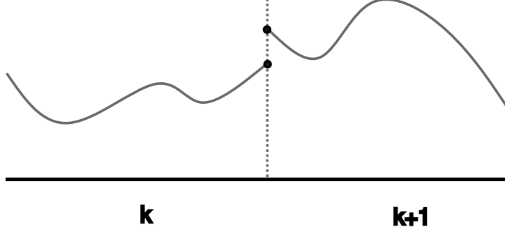
Figure 1: u_h is multivalued at the elemental interfaces
