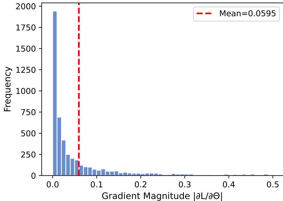
Standard BPR
