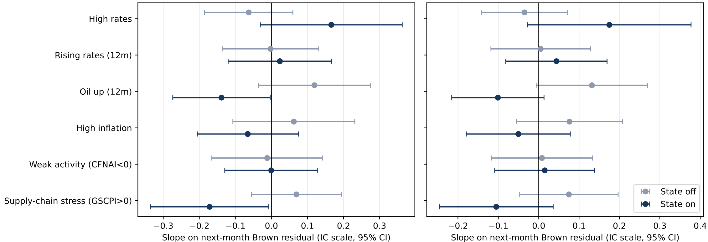
Raw attention
