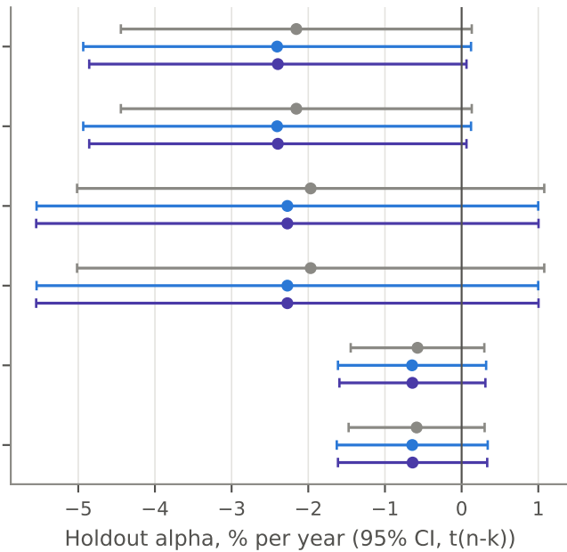
Corrected baseline
