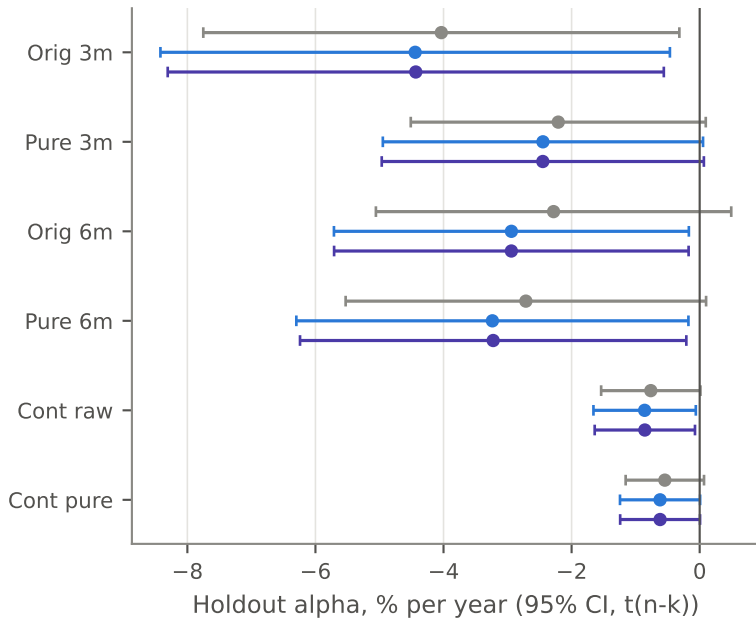
Team baseline
