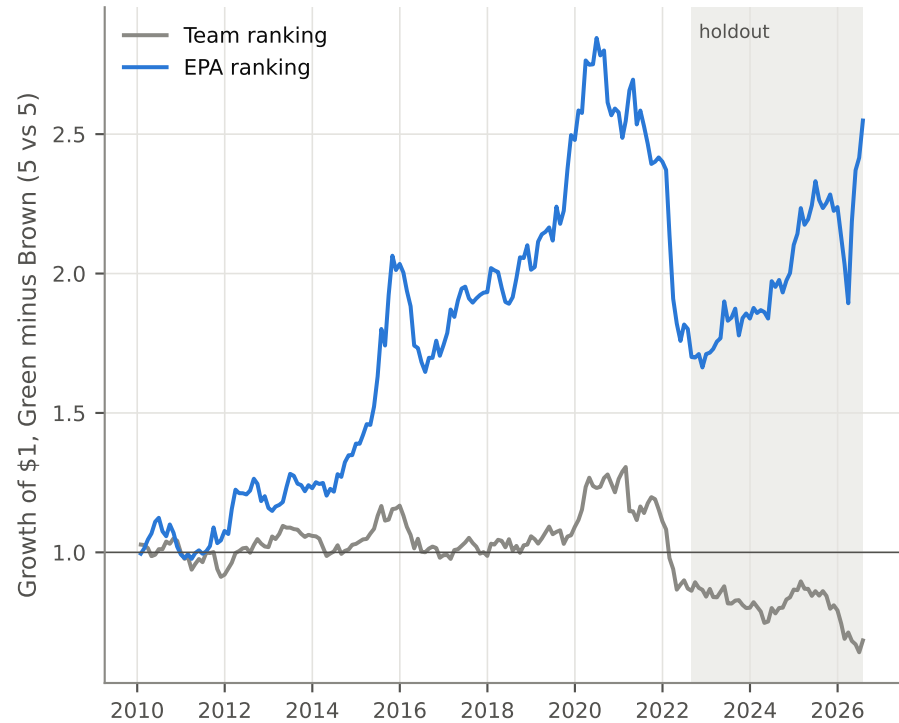
(b) Post-2010 (primary test window)
