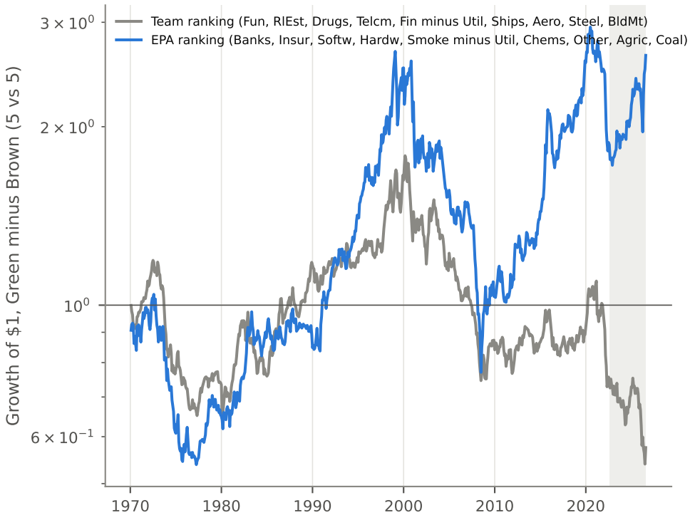
(a) 1970-01 to 2026-07 (log scale)
