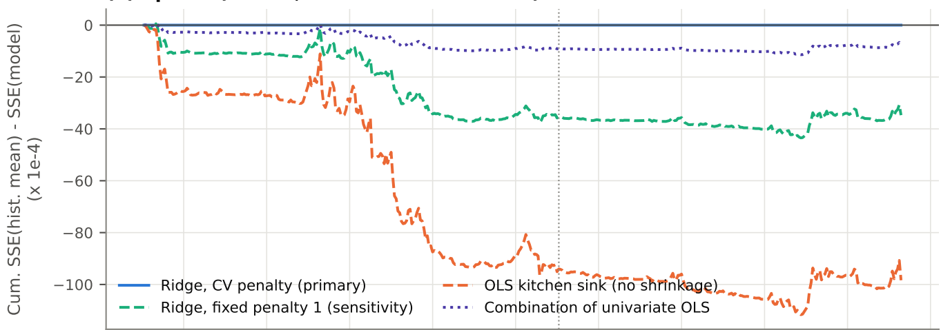
(b) Spec B (full, estimation from 1990): model vs historical mean
