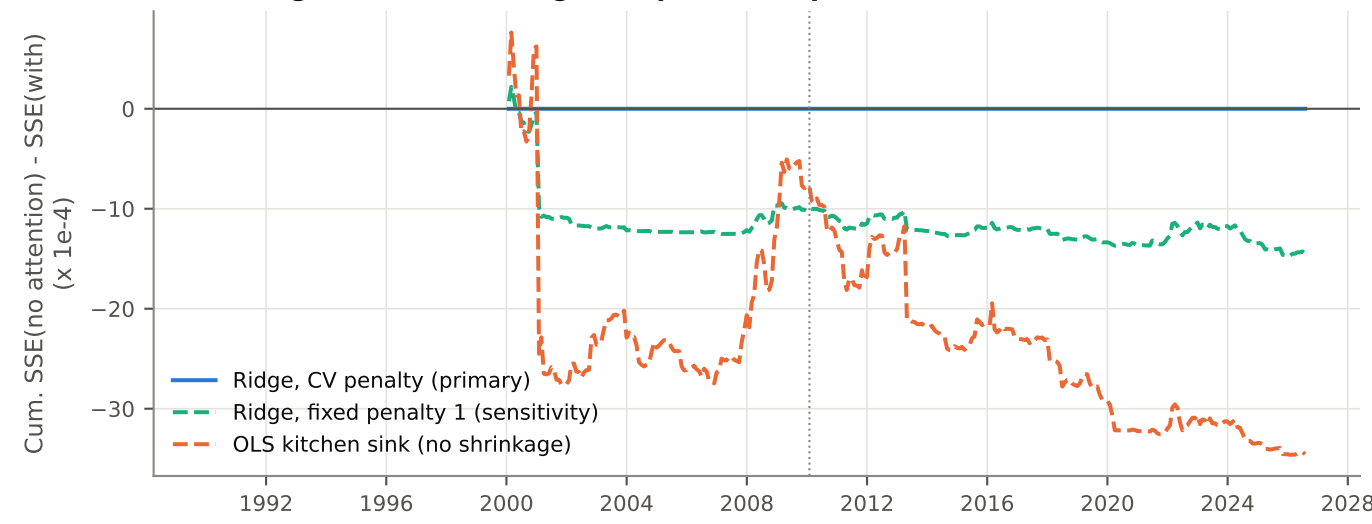
(c) Adding the attention signal: Spec B vs Spec B without attention
