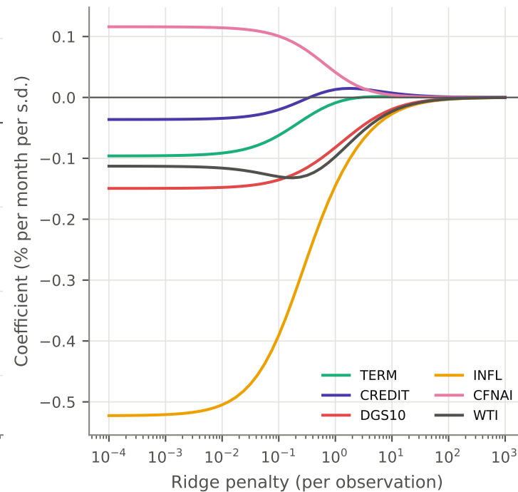
(b) Spec B: macro predictors
