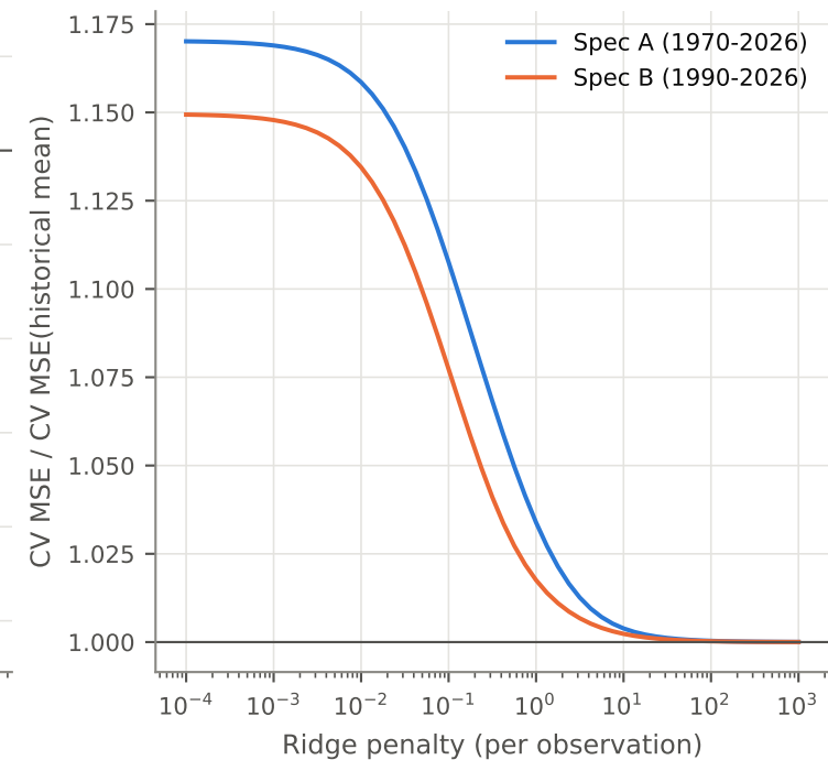
(c) CV error relative to historical mean
