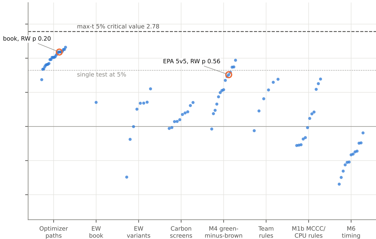
S-post: 2010-01 to 2026-07, 89 series
