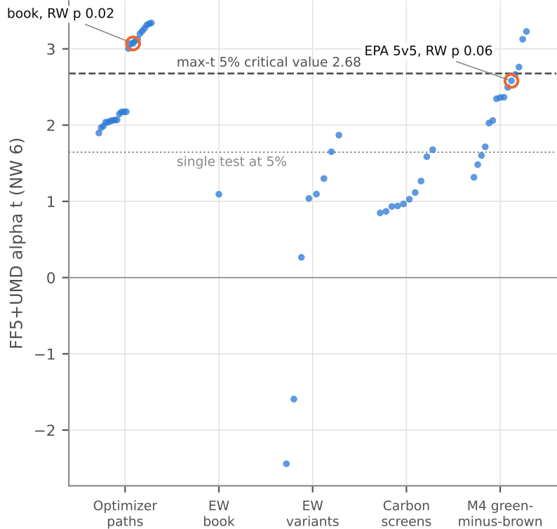
S-full: 1970-01 to 2026-07, 58 series
