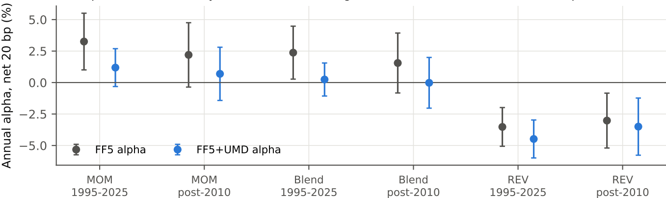
Net alpha with 95% Newey-West intervals: adding UMD removes the MOM and Blend alpha
