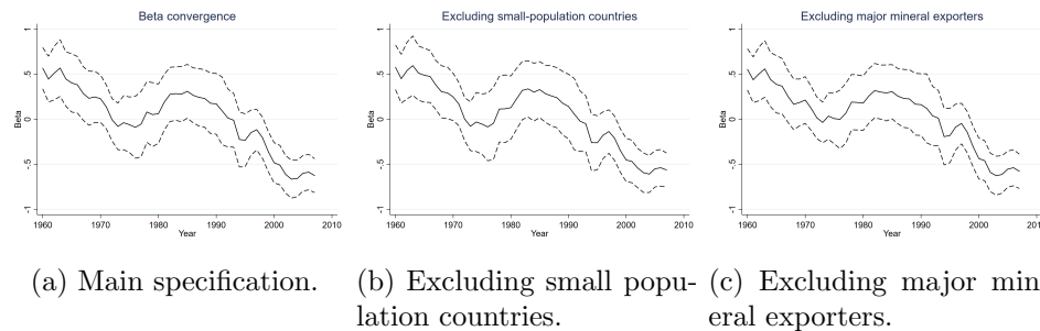
Figure A.1: Robustness of \beta -convergence to excluding small countries and major mineral exporters.
