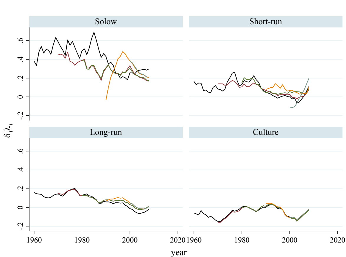
Figure A.20: Trend in difference between unconditional and conditional convergence, univariate ( \delta\lambda )
