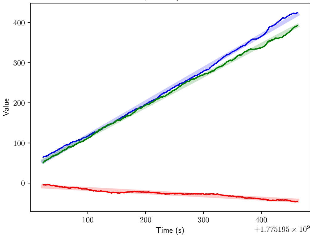
PLOT OF ROLL/PITCH/YAW LINEAR FITS
