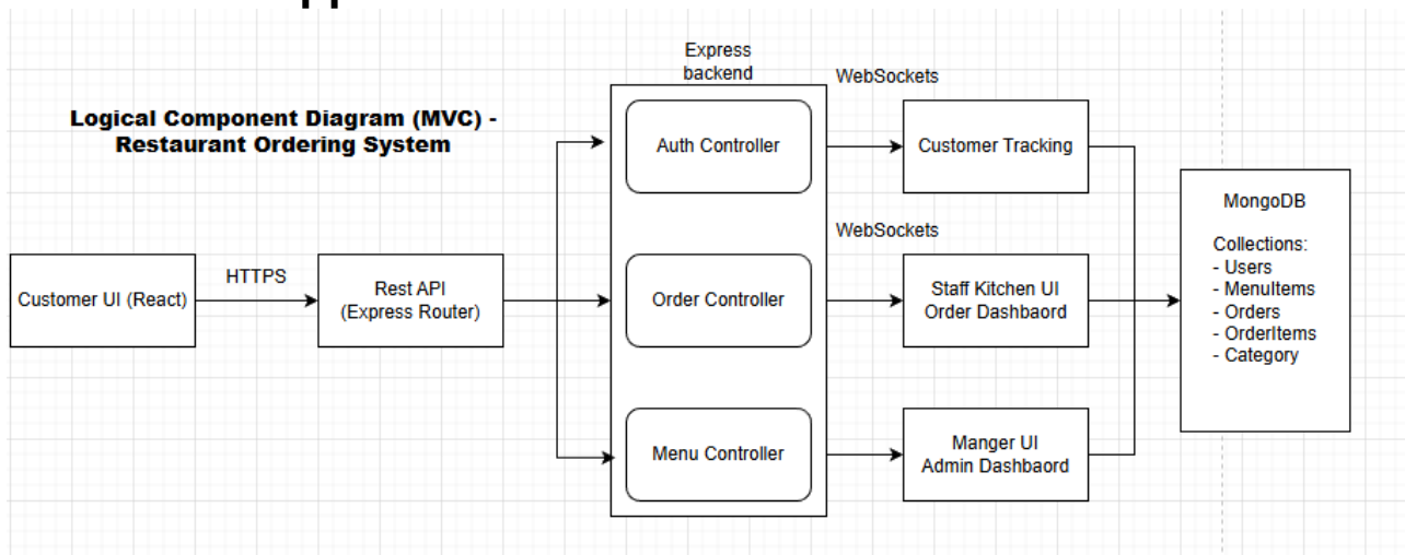
Figure 1: Component Diagram
