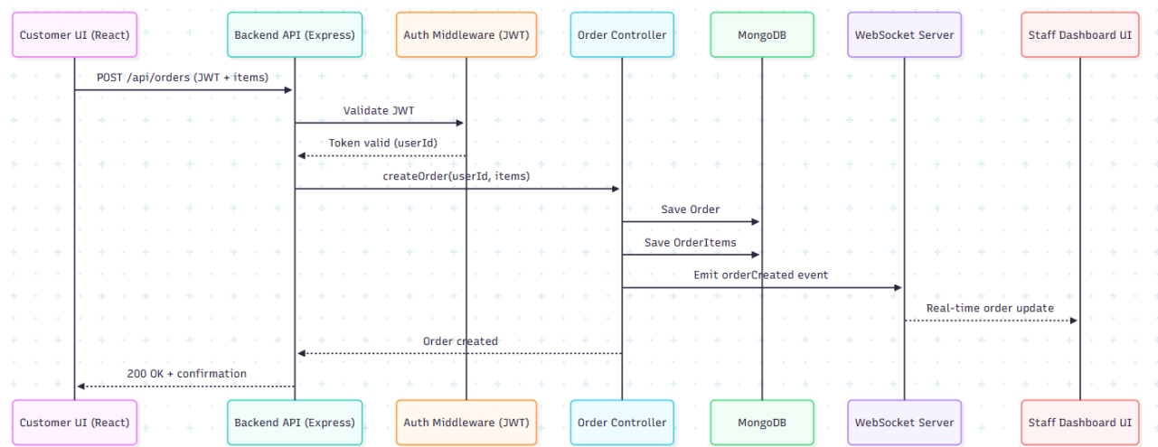
Figure 3: Sequence Diagram
