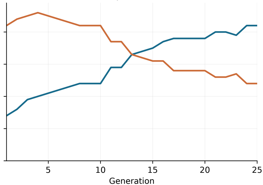
Isotropic histories
