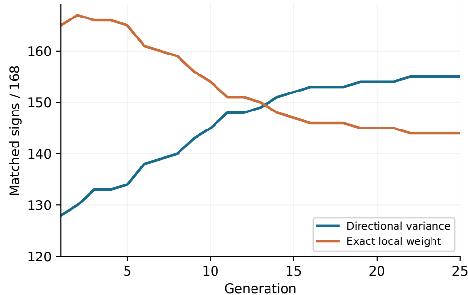
Structured histories
