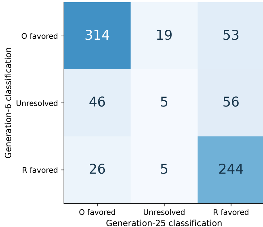
Isotropic histories (768 checkpoints)
