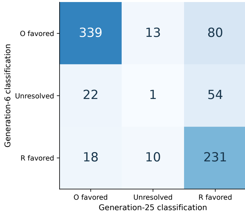
Structured histories (768 checkpoints)
