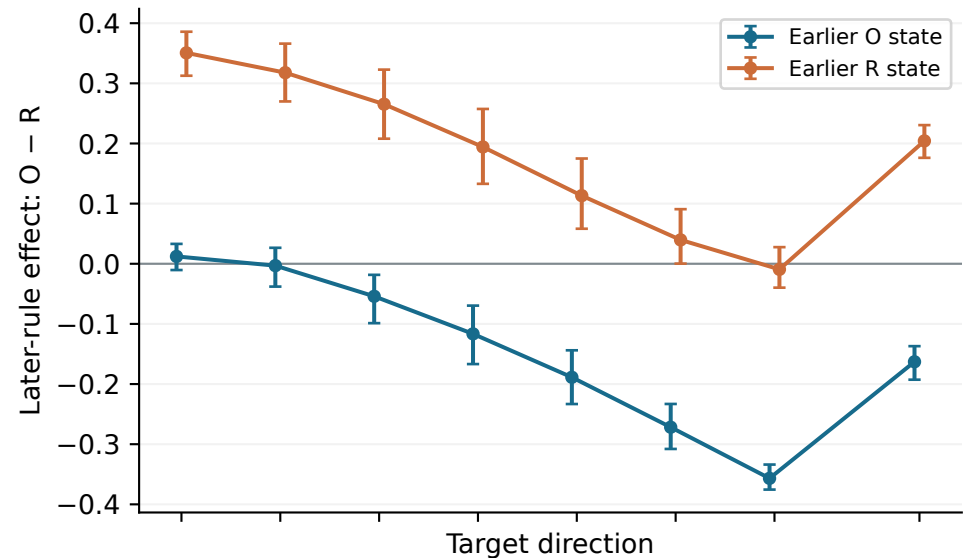
Structured histories
