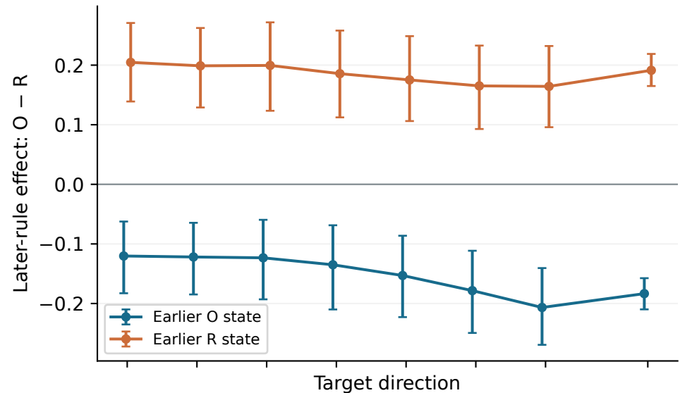
Isotropic histories
